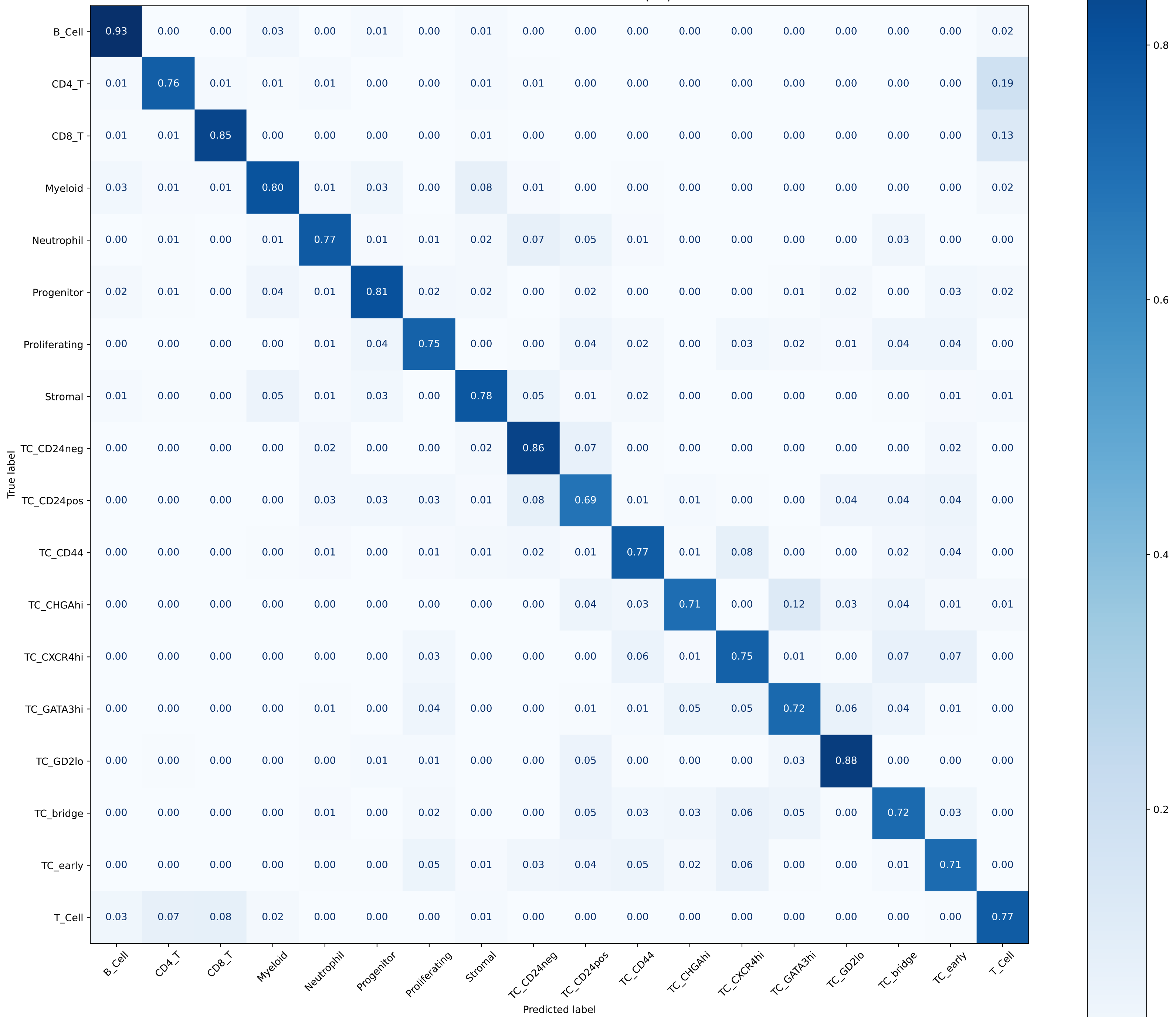
Confusion Matrix — Linear Probe (Val)
