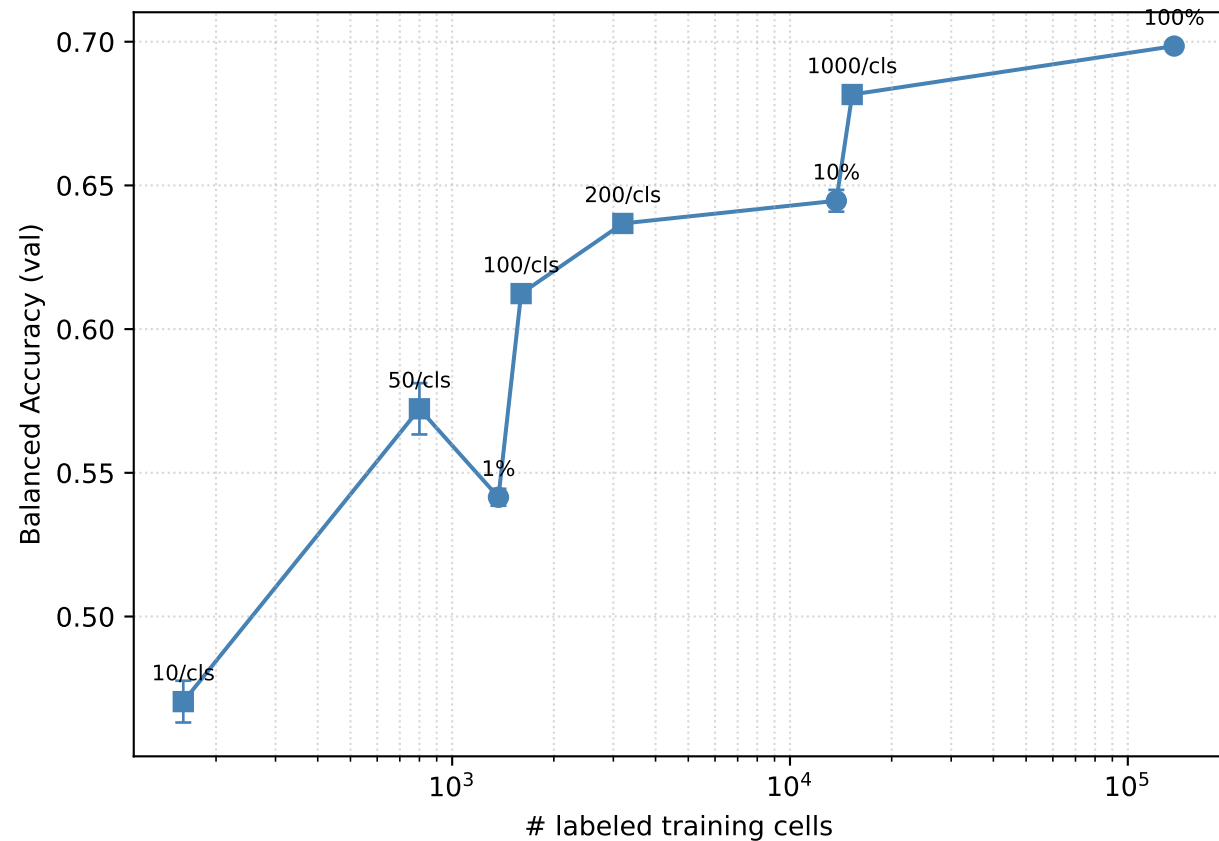
Label Efficiency — ResNet
