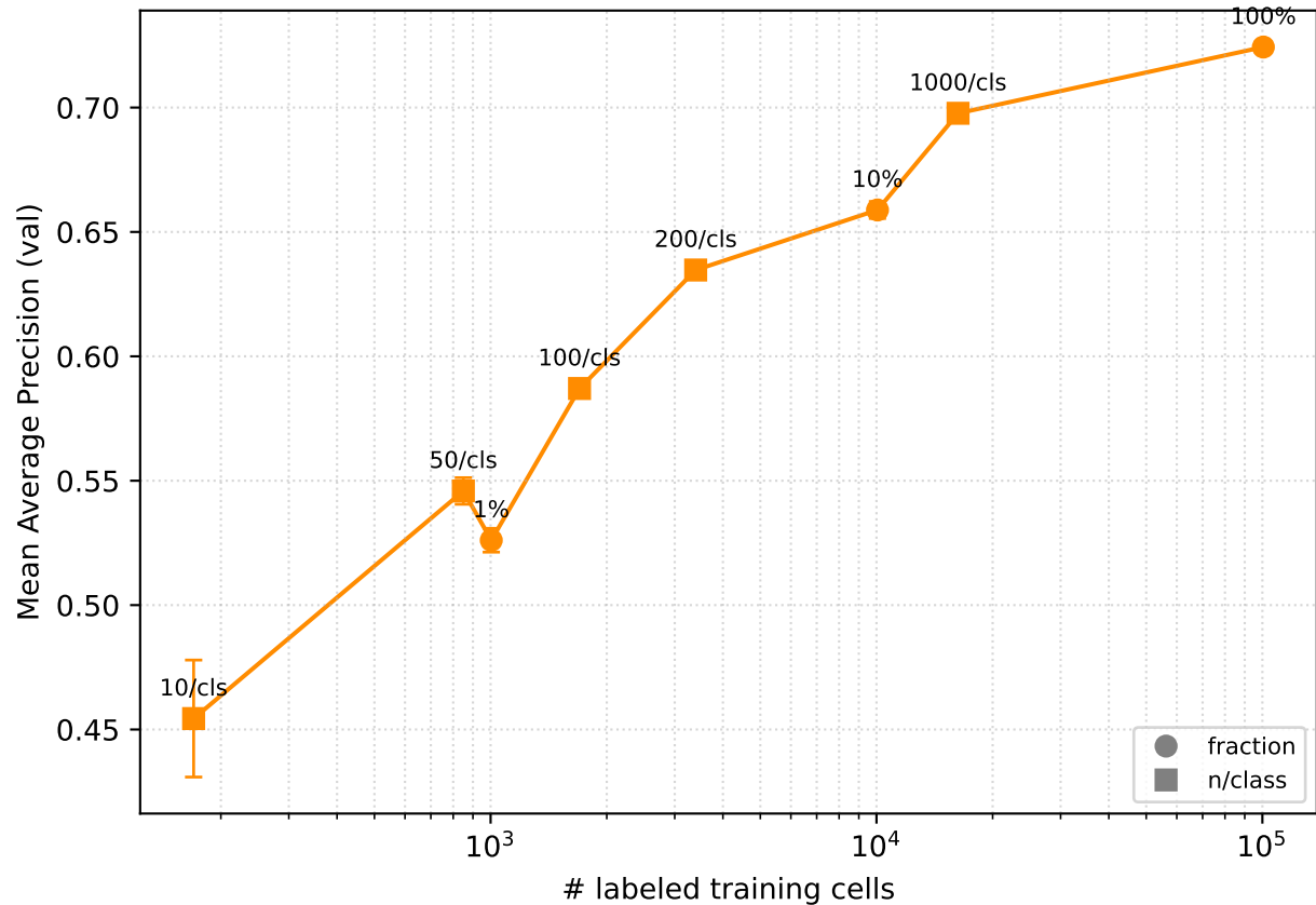
Label Efficiency — CODEX_cHL_CIM_VeryStrongAug_VICReg
