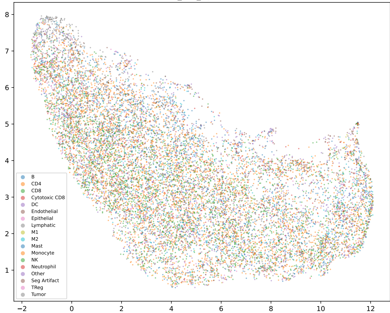
CODEX_cHL_OpenPhenom
