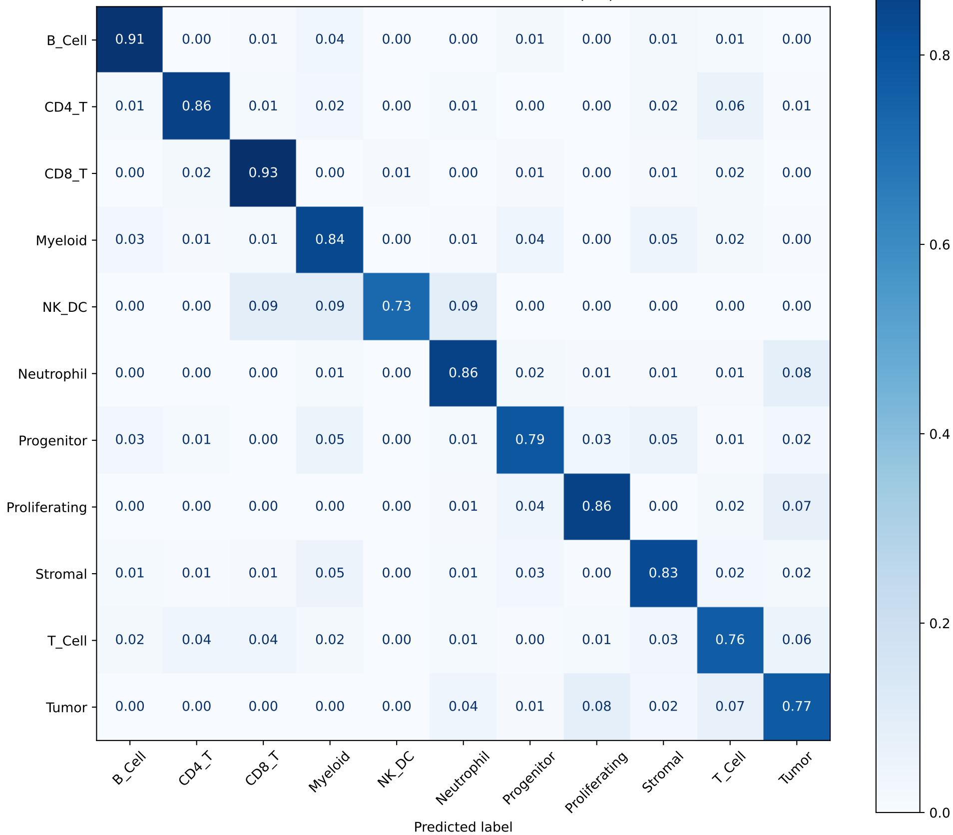
Confusion Matrix — Linear Probe (Val)
