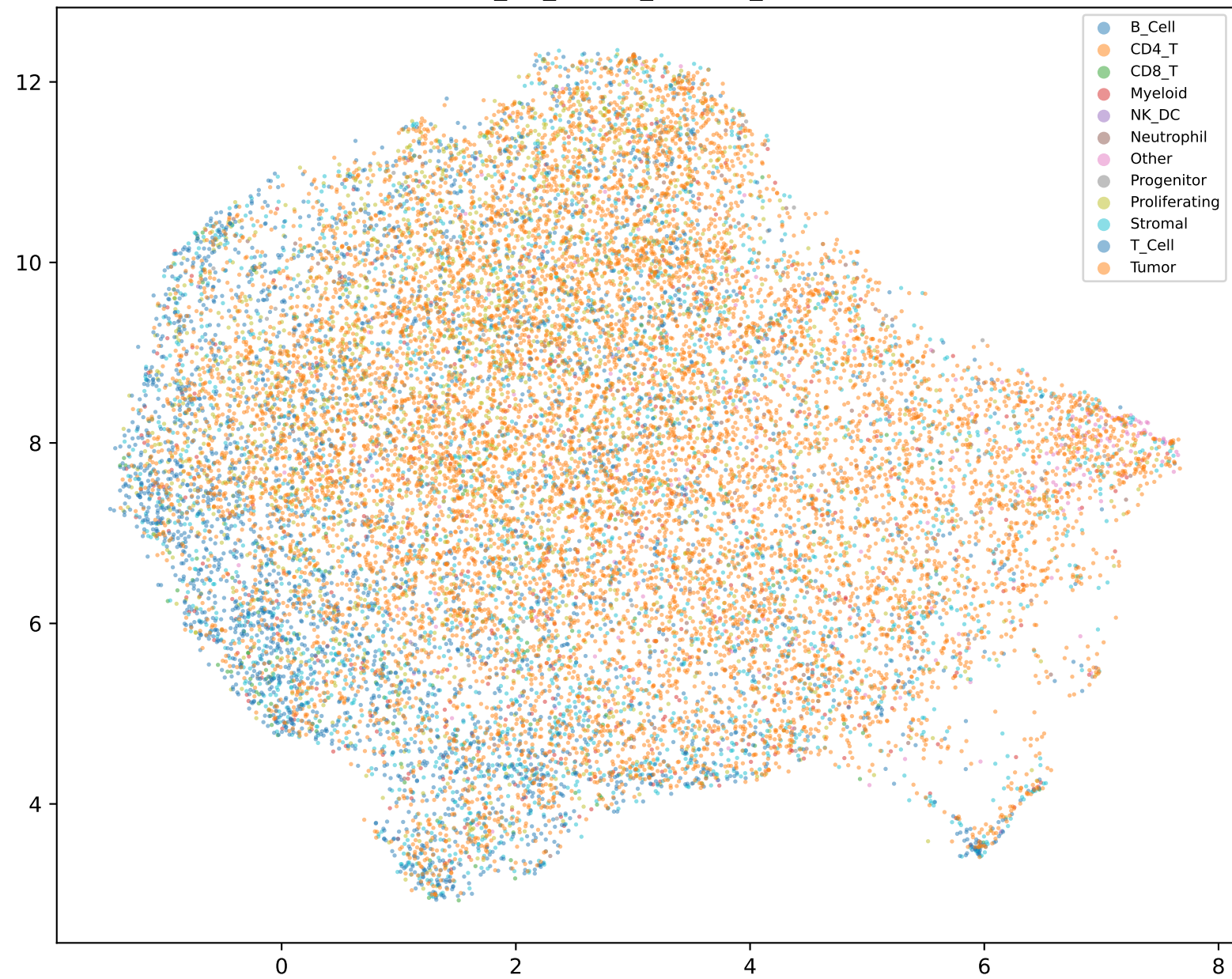
IMC_NB_FineCT_DINov2_vitb14
