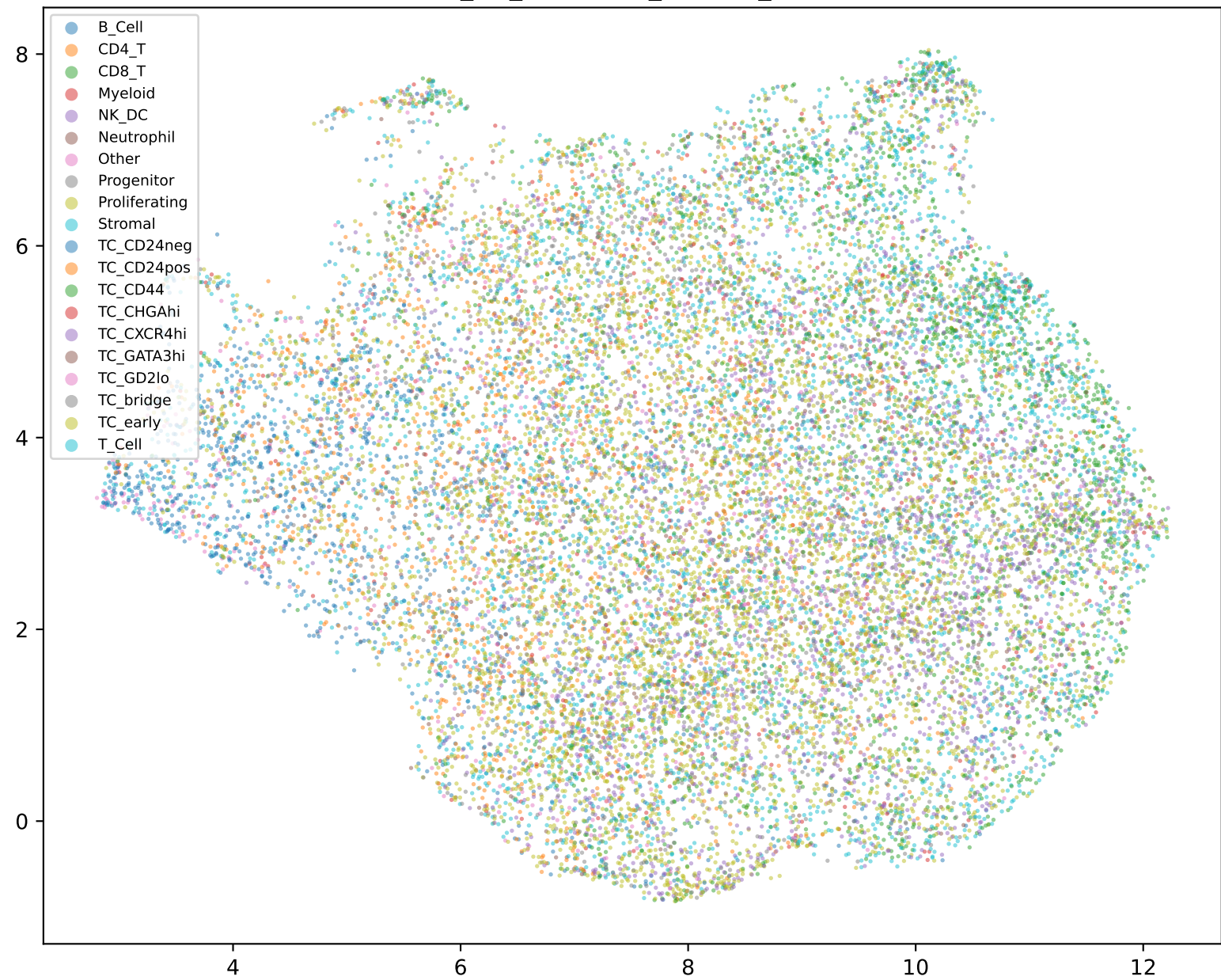
IMC_NB_TumorSub_DINOV2_vitb14
