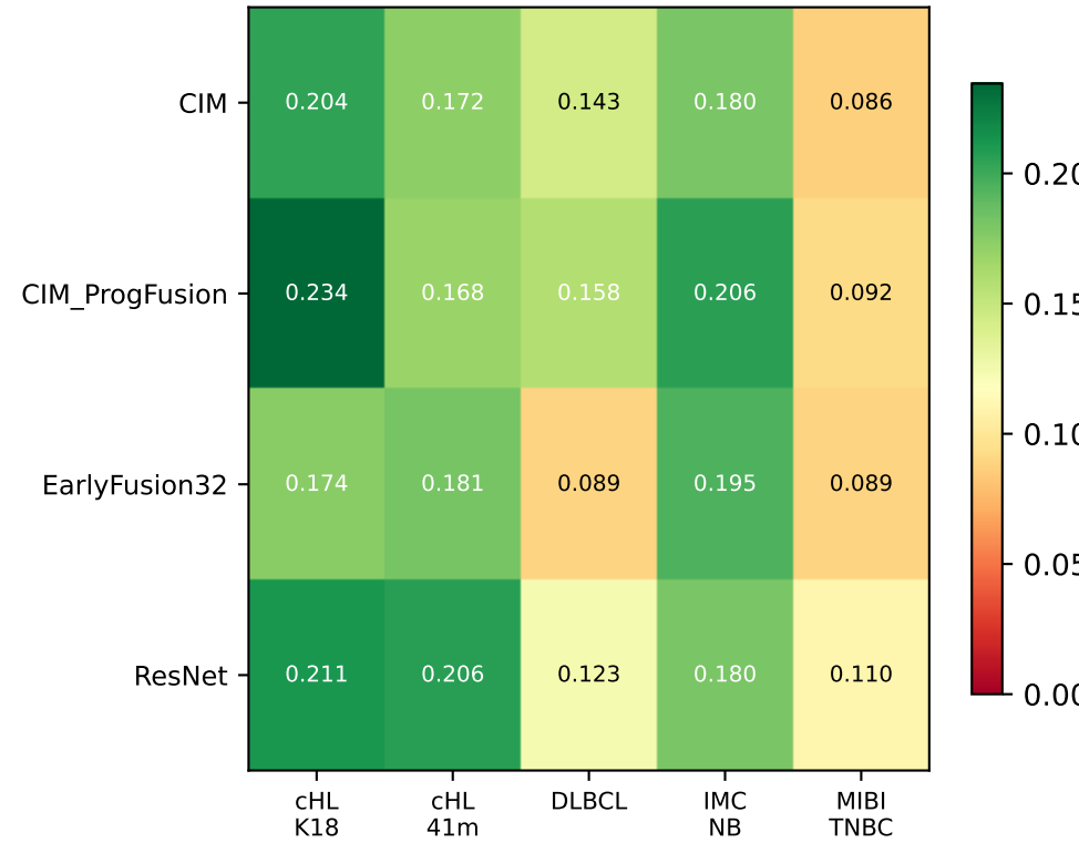
ARI
