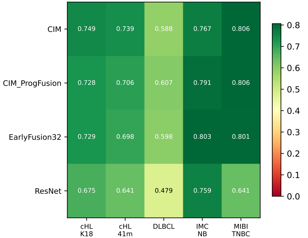
Silhouette
