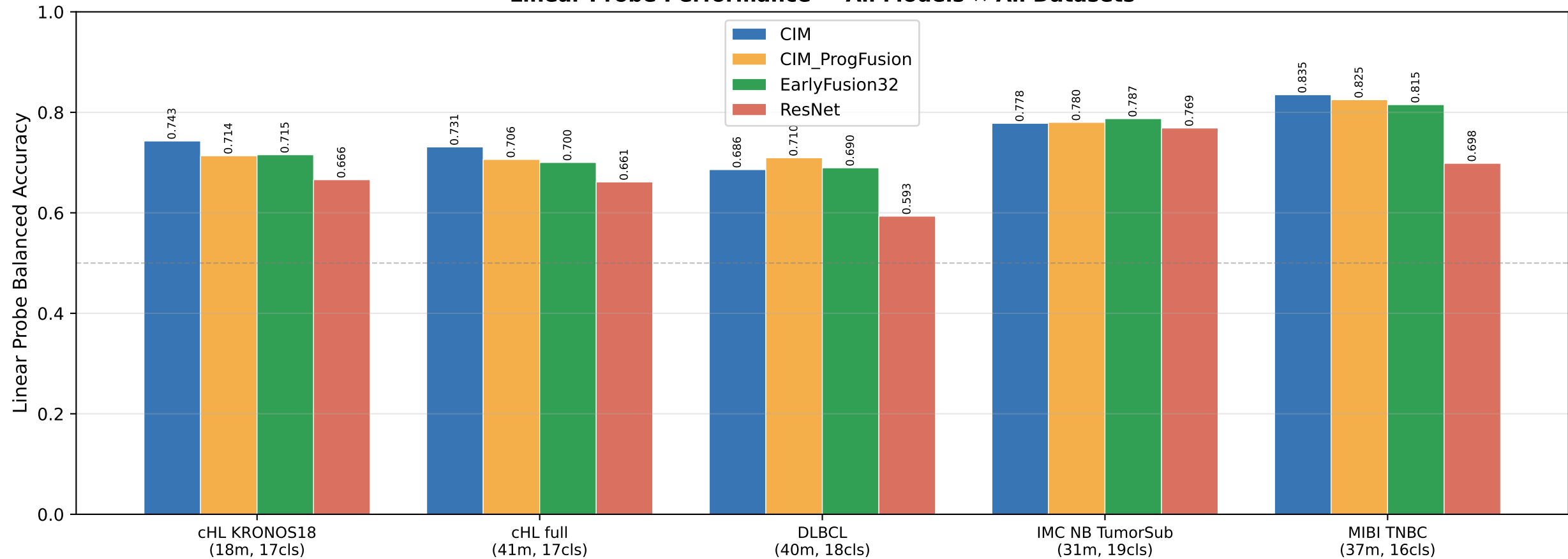
Linear Probe Performance — All Models × All Datasets
