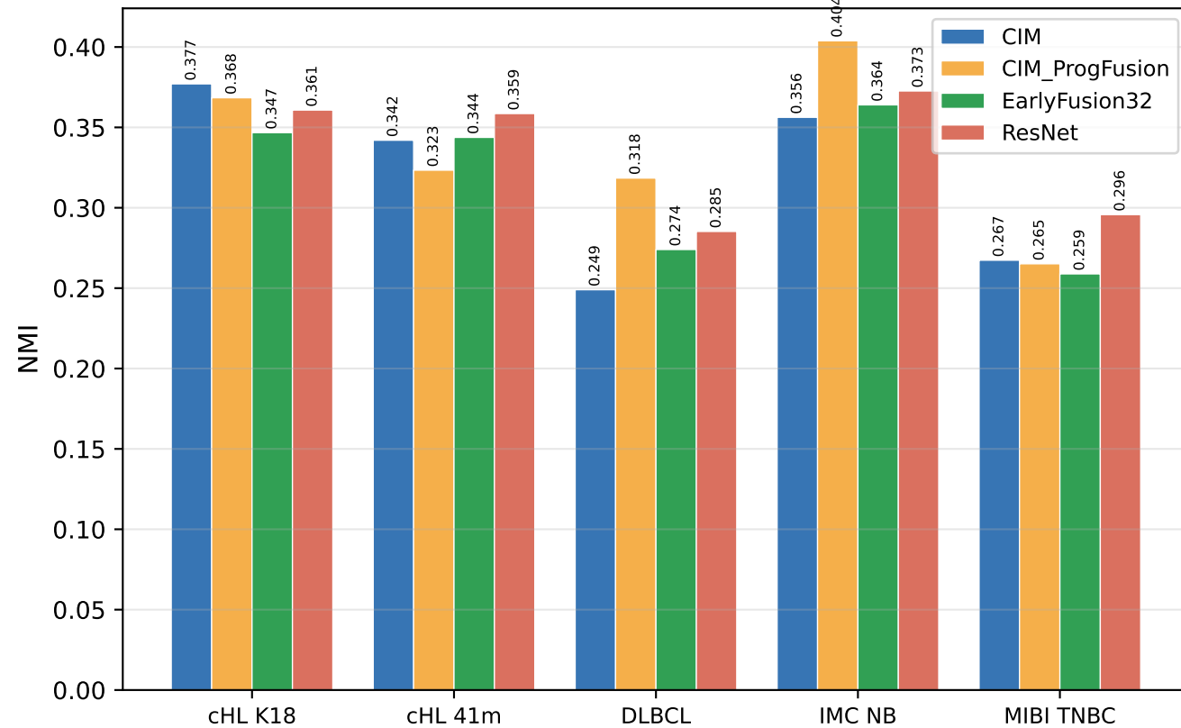
Clustering Quality — NMI
