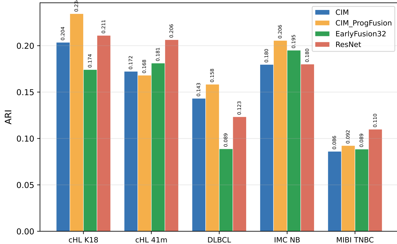
Clustering Quality — ARI
