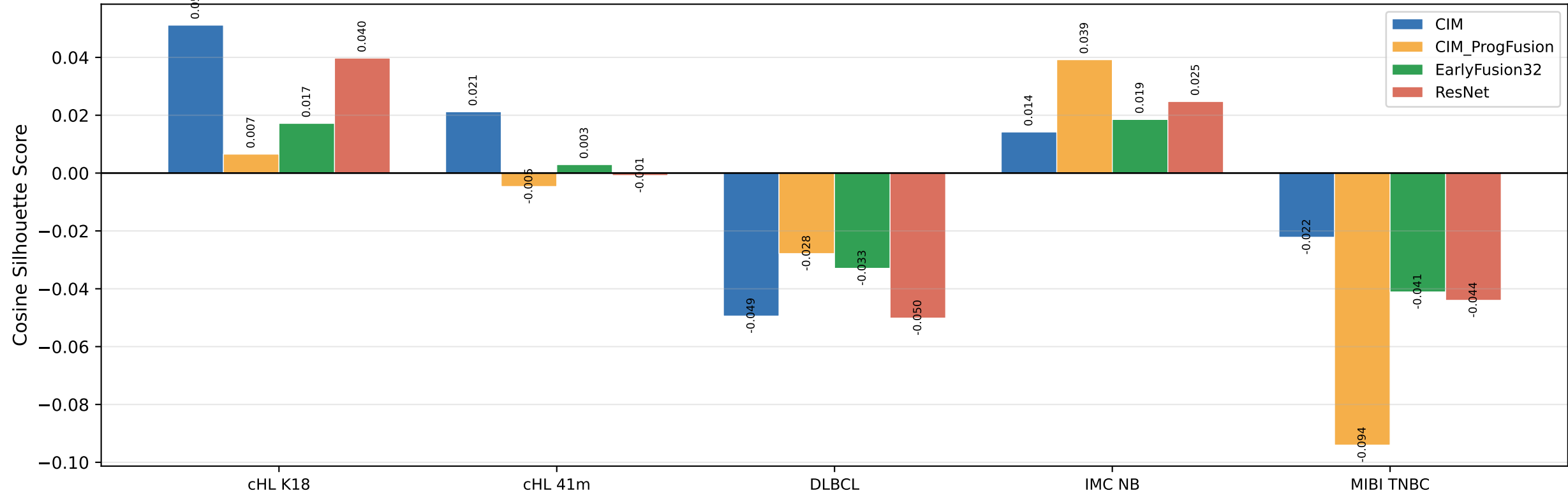
Embedding Geometry — Cosine Silhouette (positive = compact clusters)
