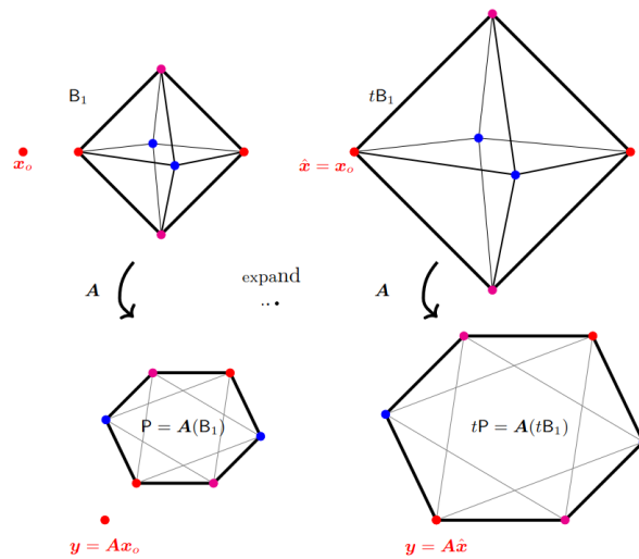
Figure 3.3: \ell_1 minimization in the observation-space.
