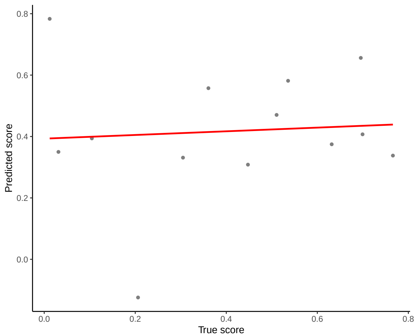
Predicted vs True (Test)
