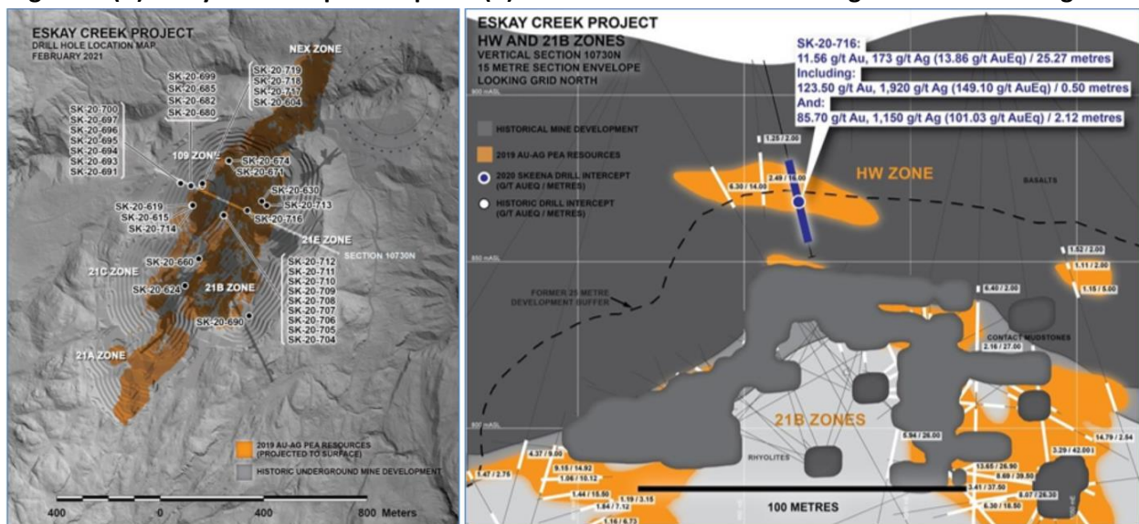
Figure 1: (A) Eskay drill hole plan map and (B) vertical section 10730N through Zone 21B looking north
