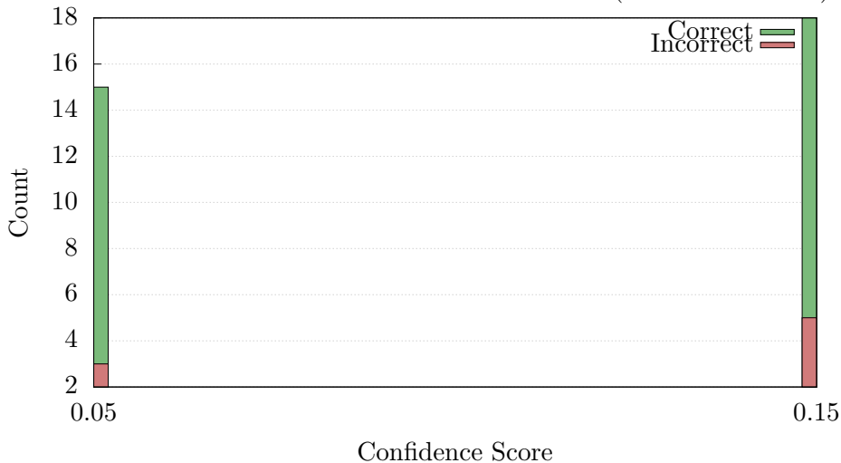
Confidence Distribution: Correct vs Incorrect (Norm-Shift Head)
