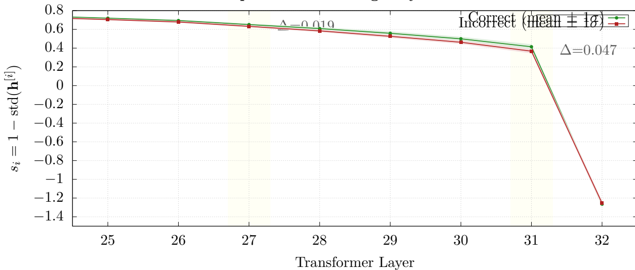
Separation Widening: Layers 25–32
