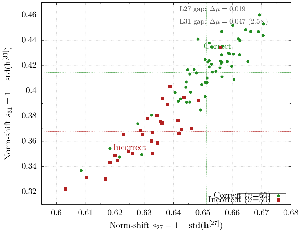
Confidence Head: Layer 27 vs Layer 31 Norm-Shift Separation
