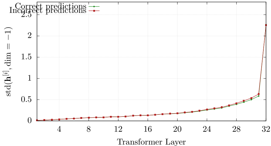
Hidden State \text{std}(\mathbf{h}^{[i]}) by Layer — Llama-3.1-8B
