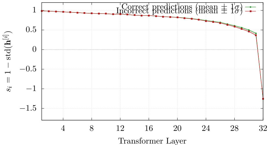
Norm-Shift Signal by Layer — Correct vs Incorrect Predictions
