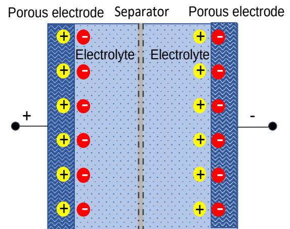
Figure 10a: Supercapacitor construction
