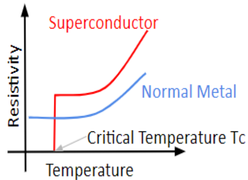
Figure 1: Resistivity Vs temperature
