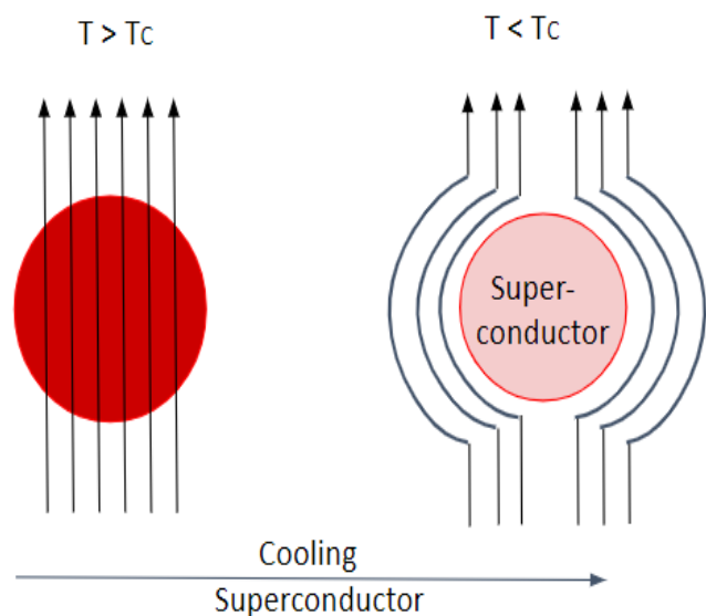
Figure 4: Meissner Effect
