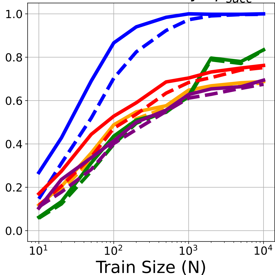
Success Probability, p_{succ}^{(n, \hat{s}^*)}
