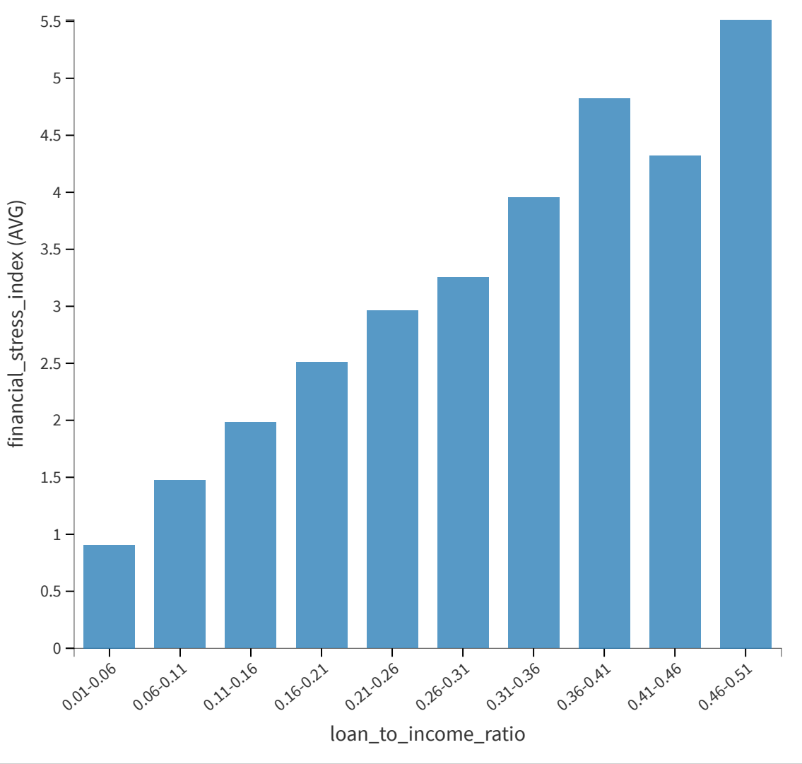
Avg of financial_stress_index by loan_to_income_ratio on credit_risk_dataset_500_final
