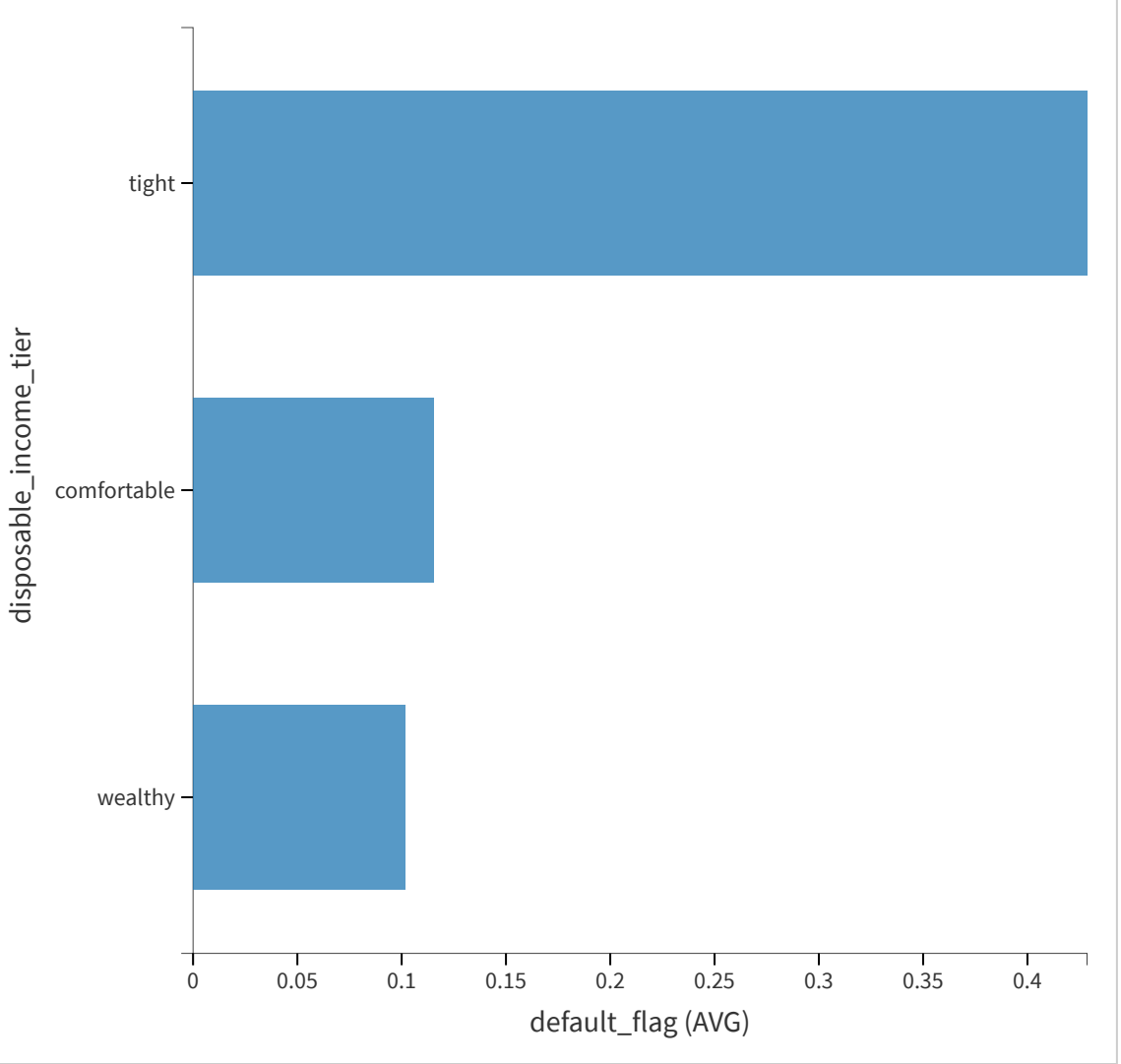
Avg of default_flag by disposable_income_tier on credit_risk_dataset_500_final
