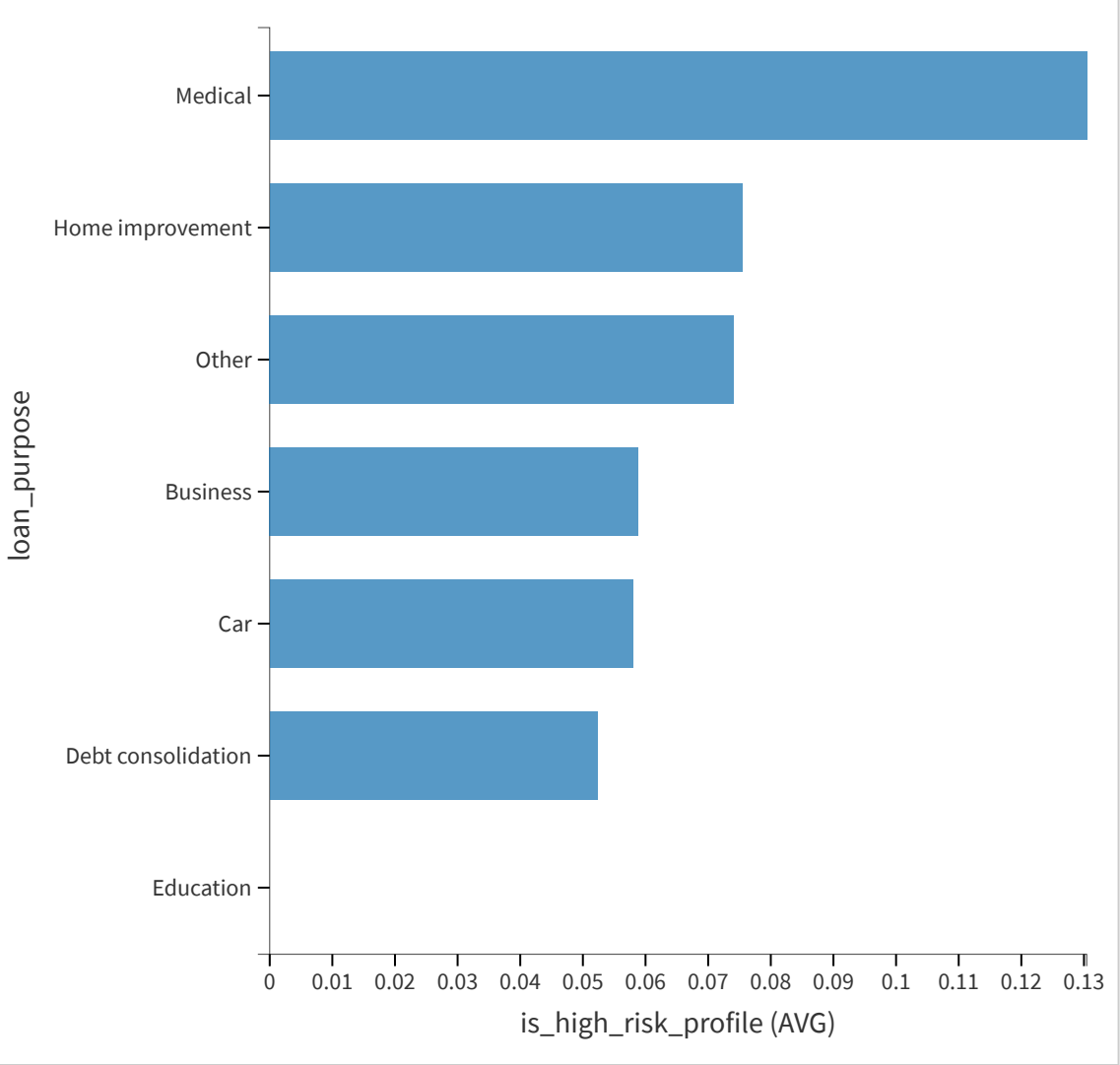
Avg of is_high_risk_profile by loan_purpose on credit_risk_dataset_500_final
