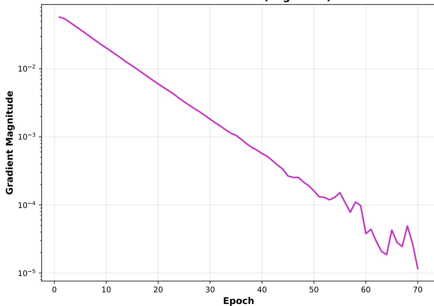
Optimization Trajectory
