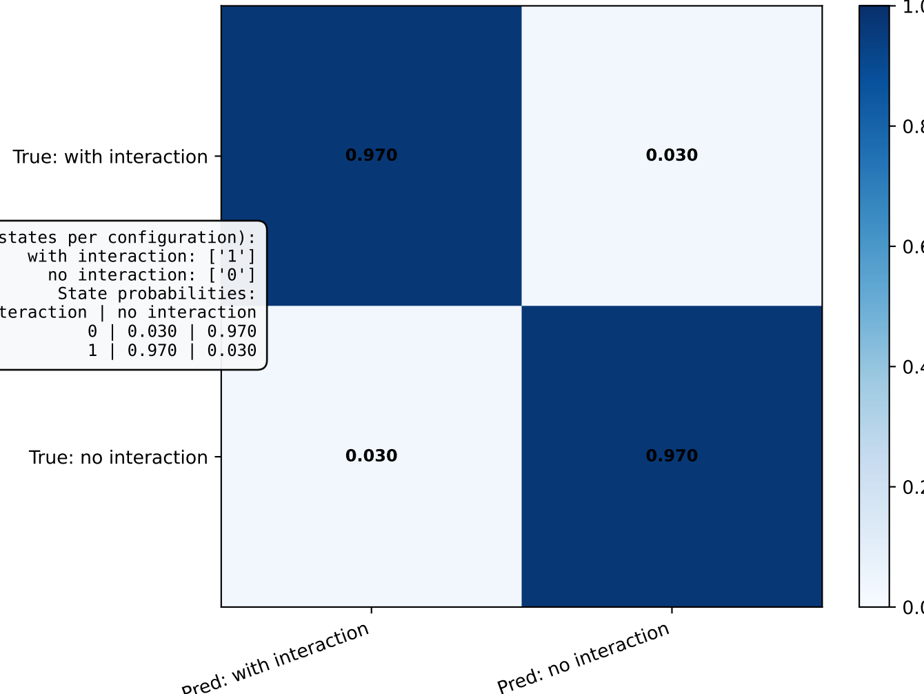
Confusion Matrix
