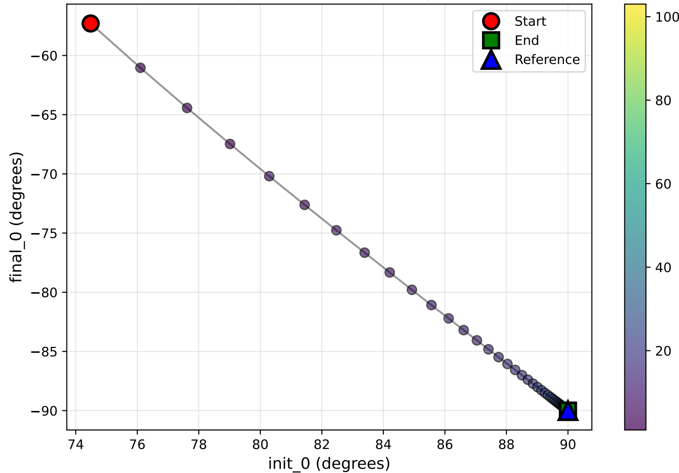
Optimization Trajectory
