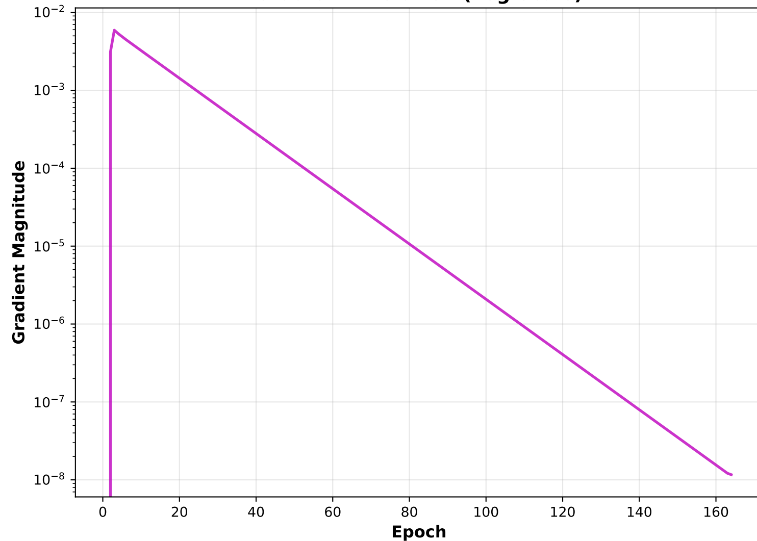
Optimization Trajectory
