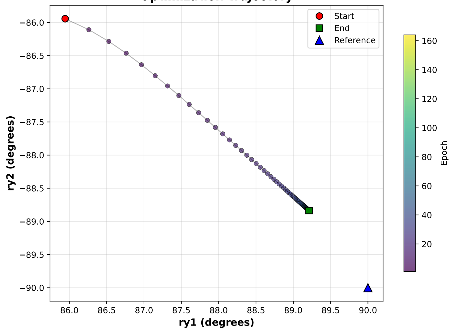
Optimization Trajectory
