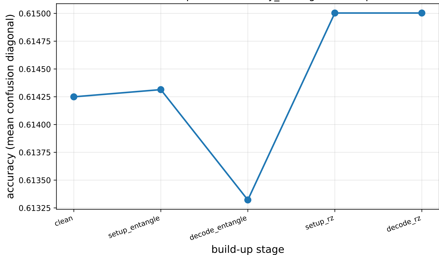
Coherent-drive 2-qubit detector: 'ry_entangle' build-up chain
