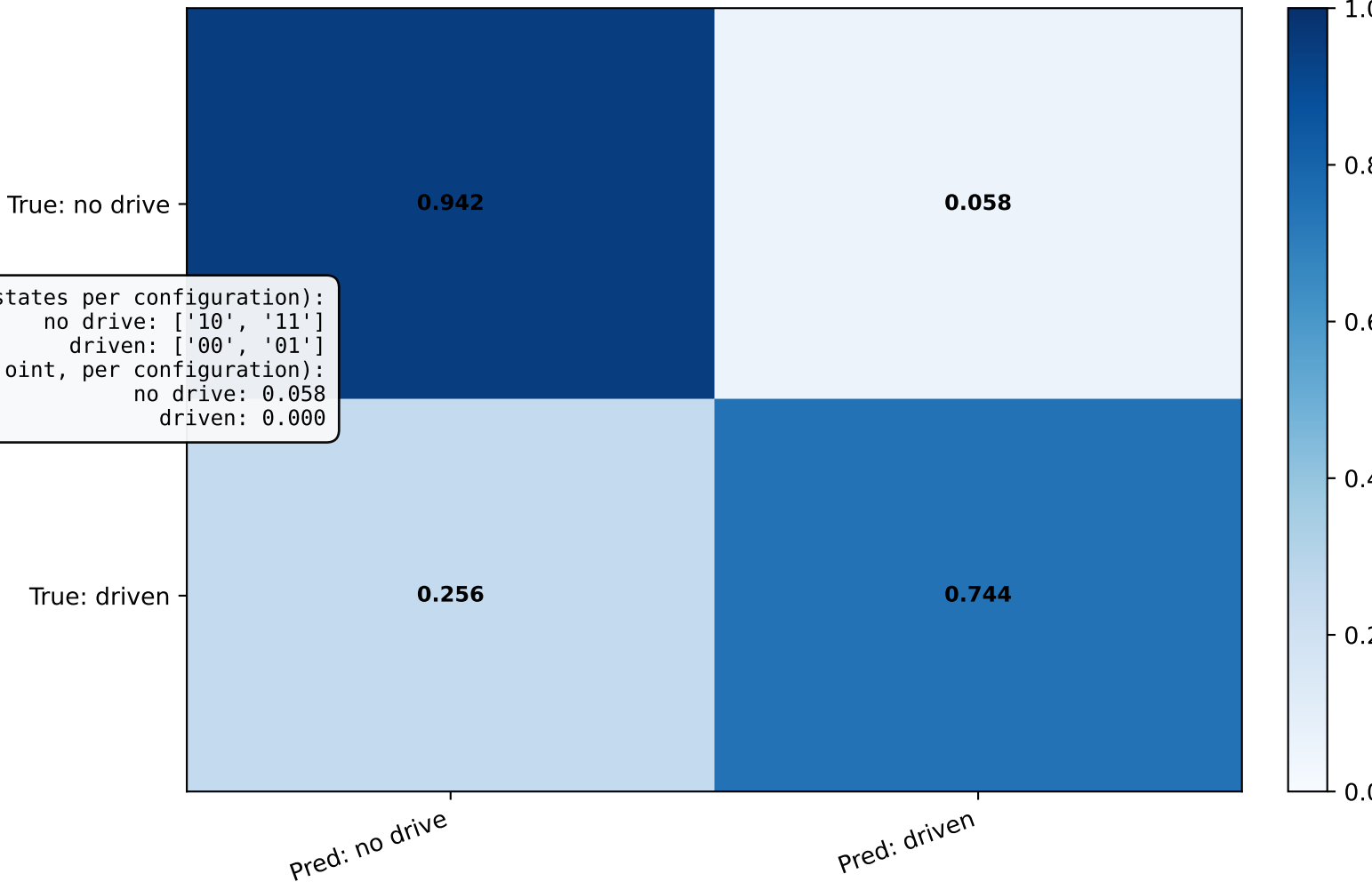
Confusion Matrix
