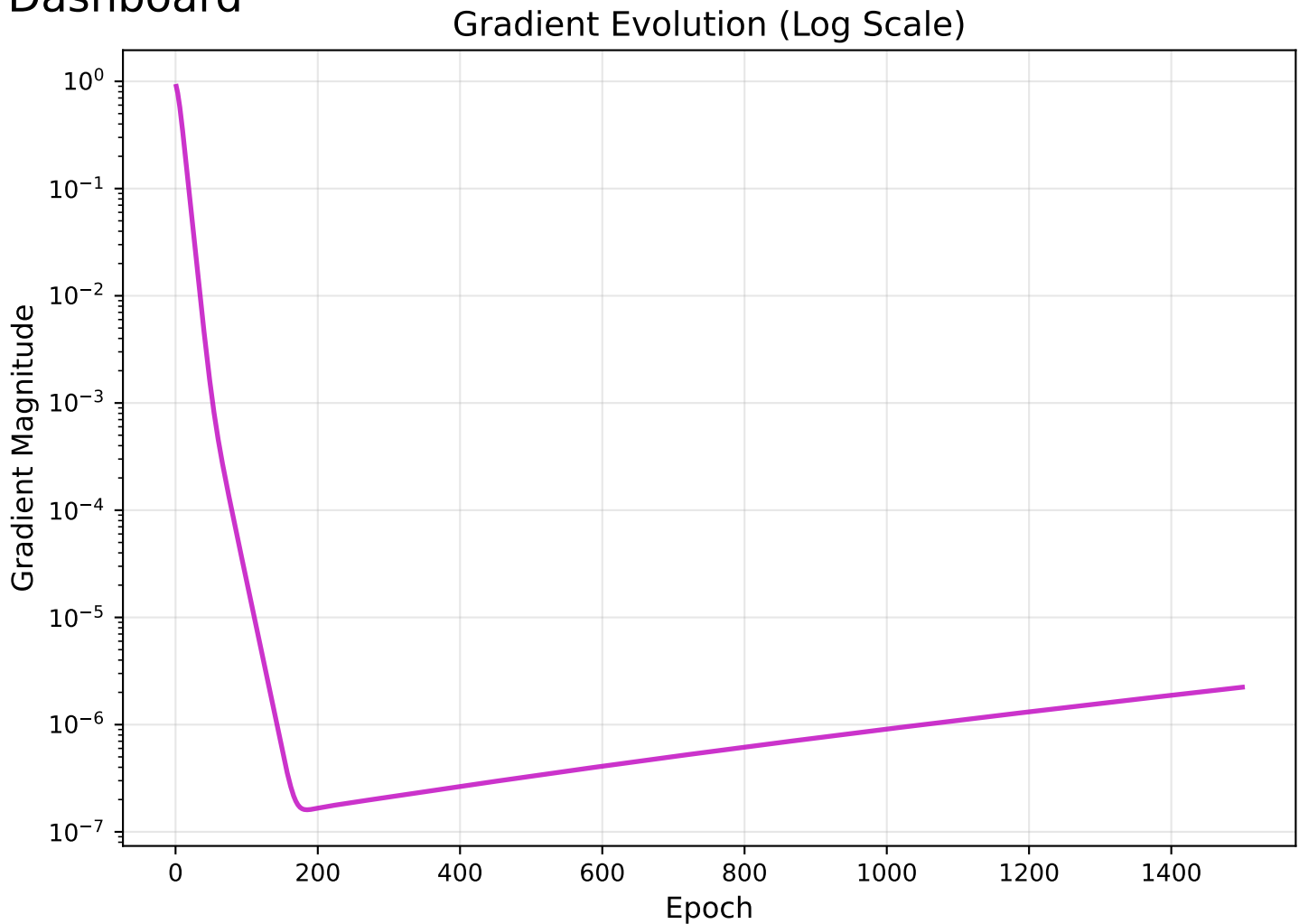
Optimization Dashboard
