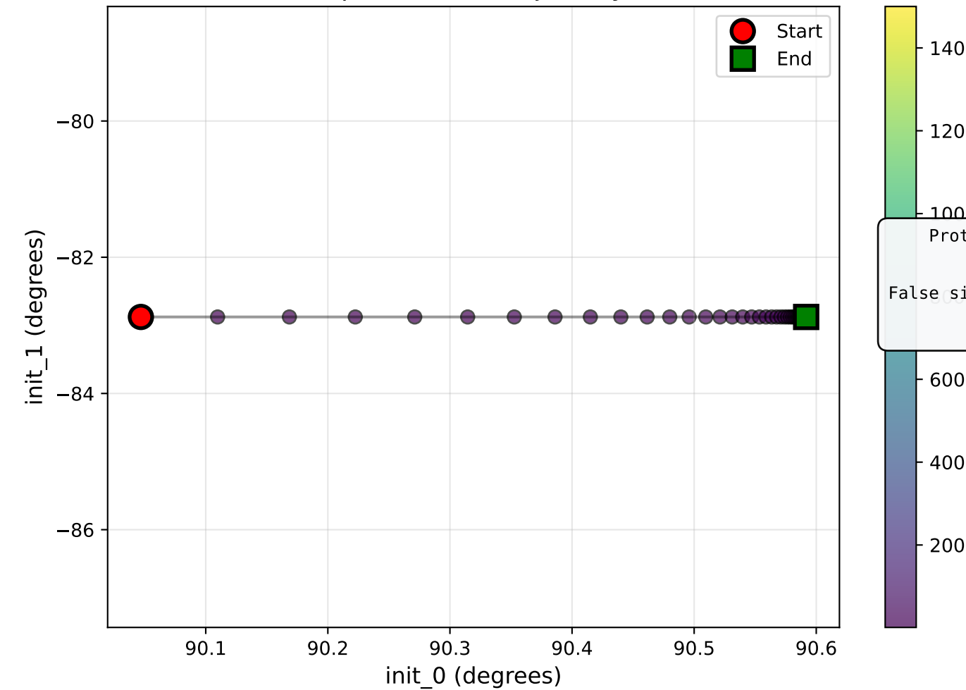
Optimization Trajectory
