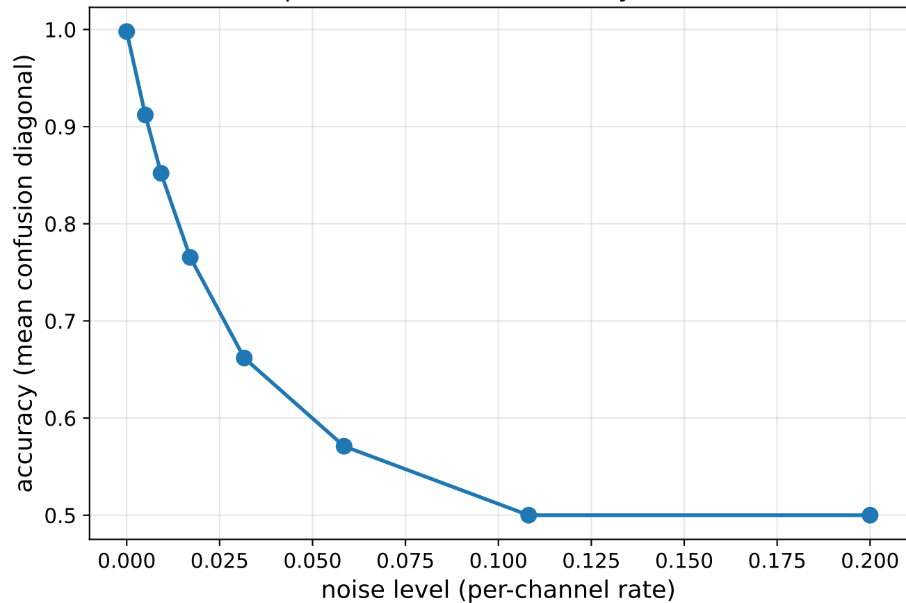
1-qubit RY detector: accuracy vs noise
