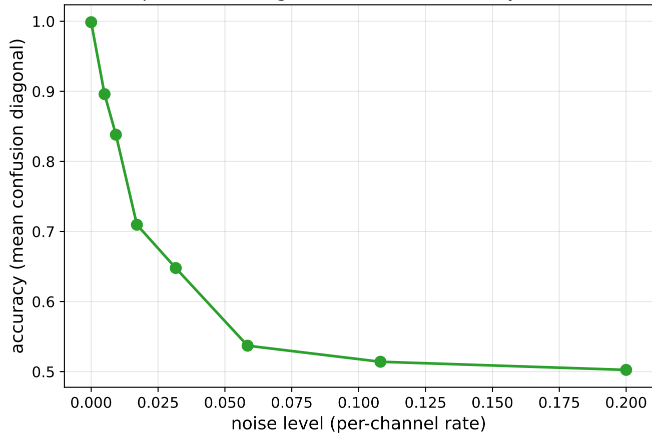
2-qubit rot-entangle-rot detector: accuracy vs noise
