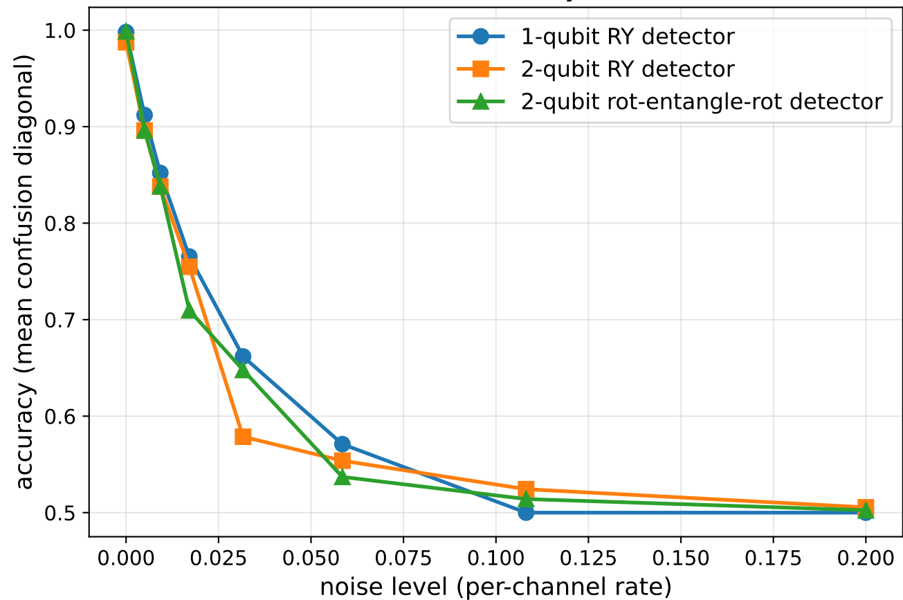
RY detector: accuracy vs noise
