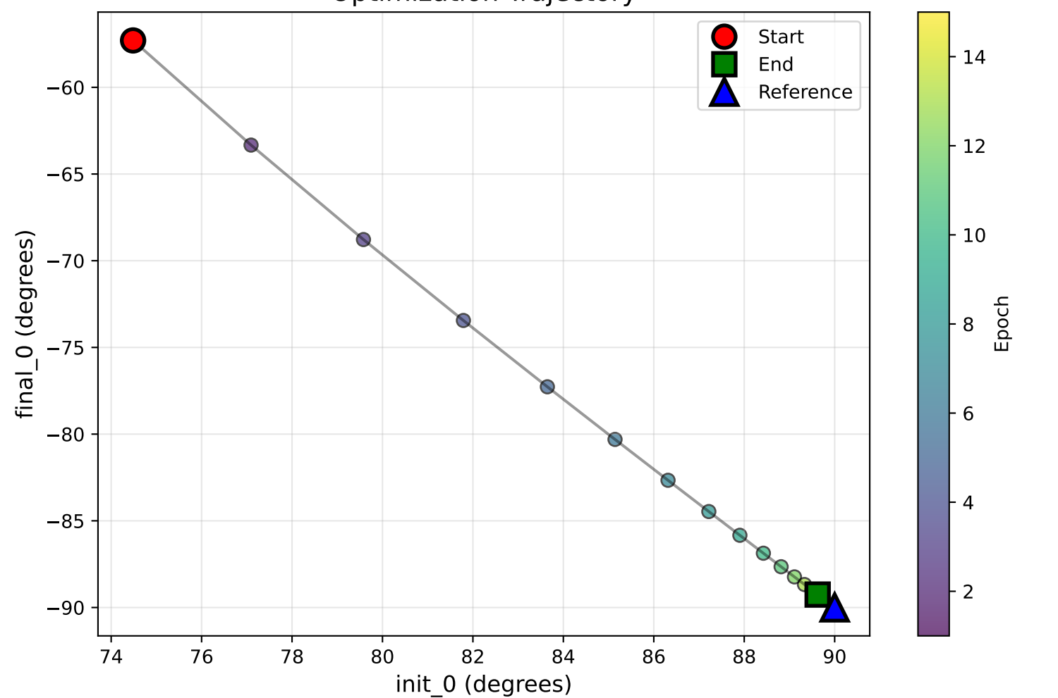
Optimization Trajectory
