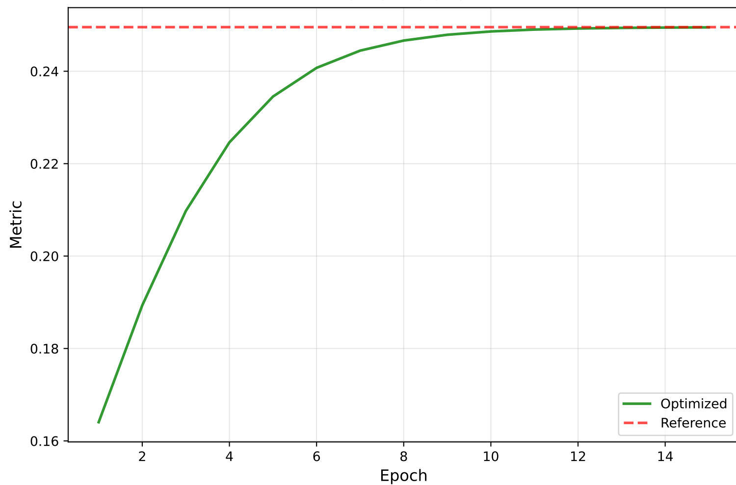
Metric Evolution
