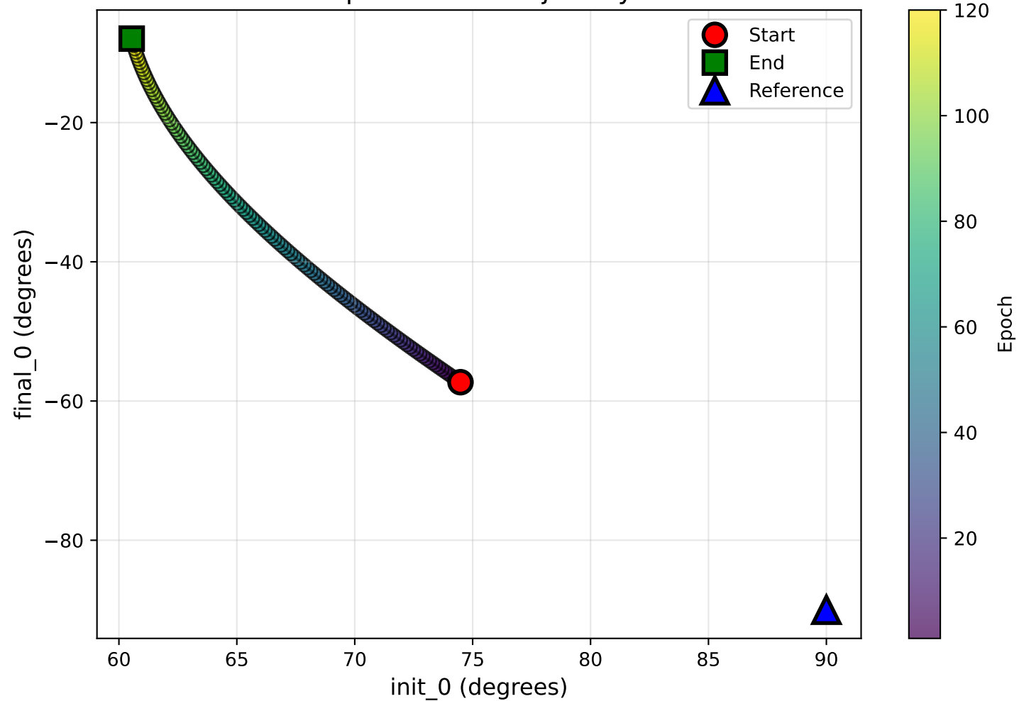
Optimization Trajectory
