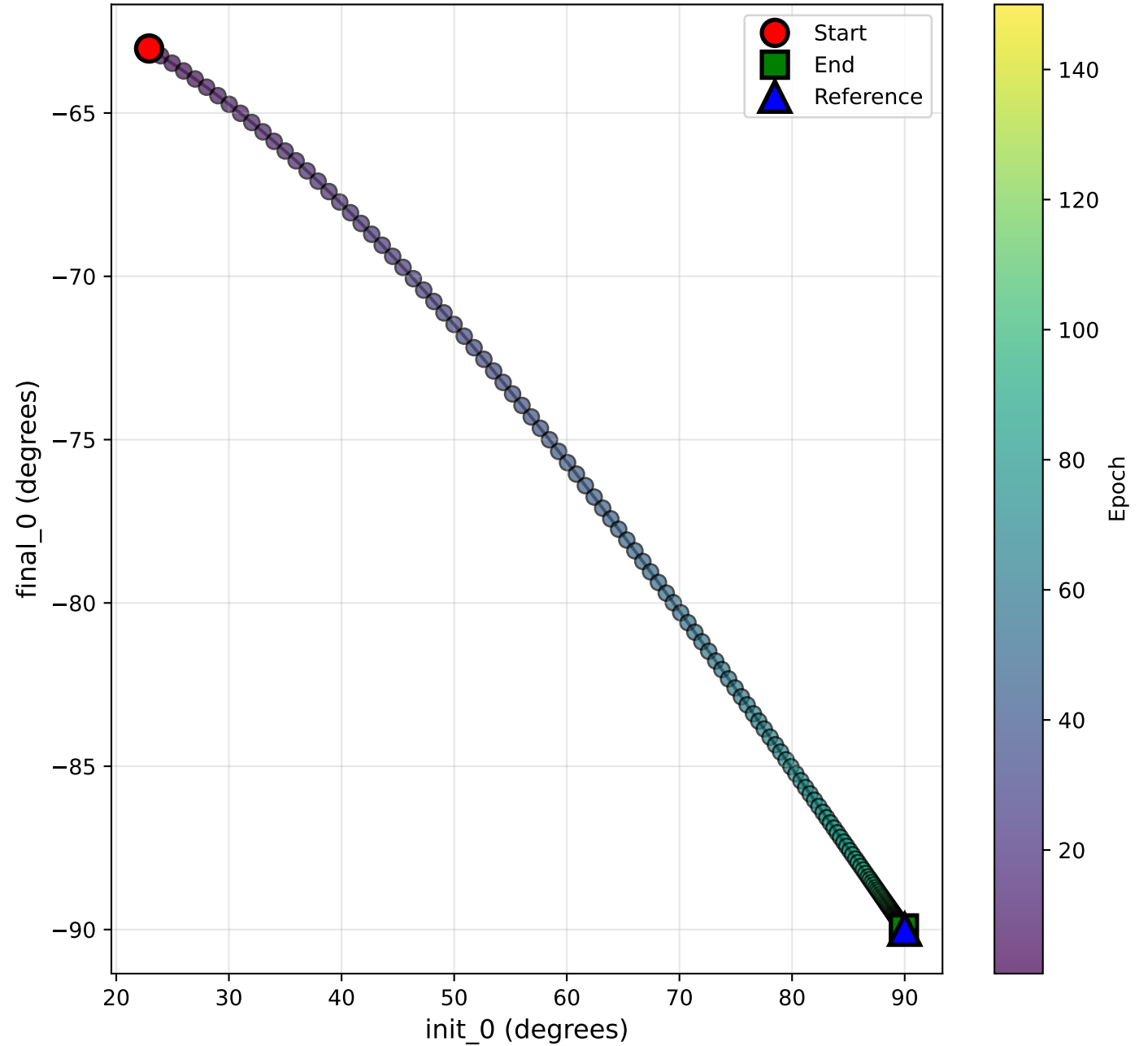
Optimization Trajectory
