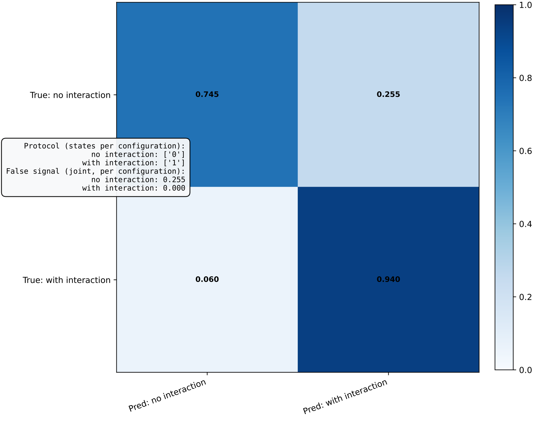
Confusion Matrix
