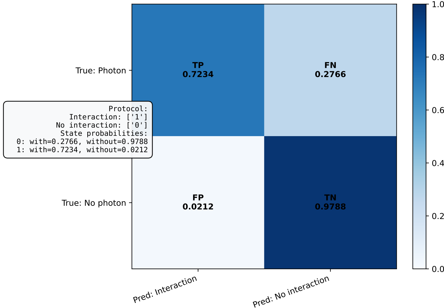
Confusion Matrix
