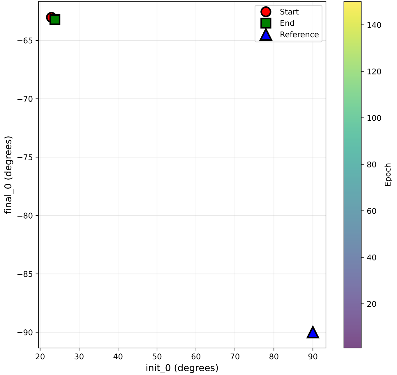
Optimization Trajectory
