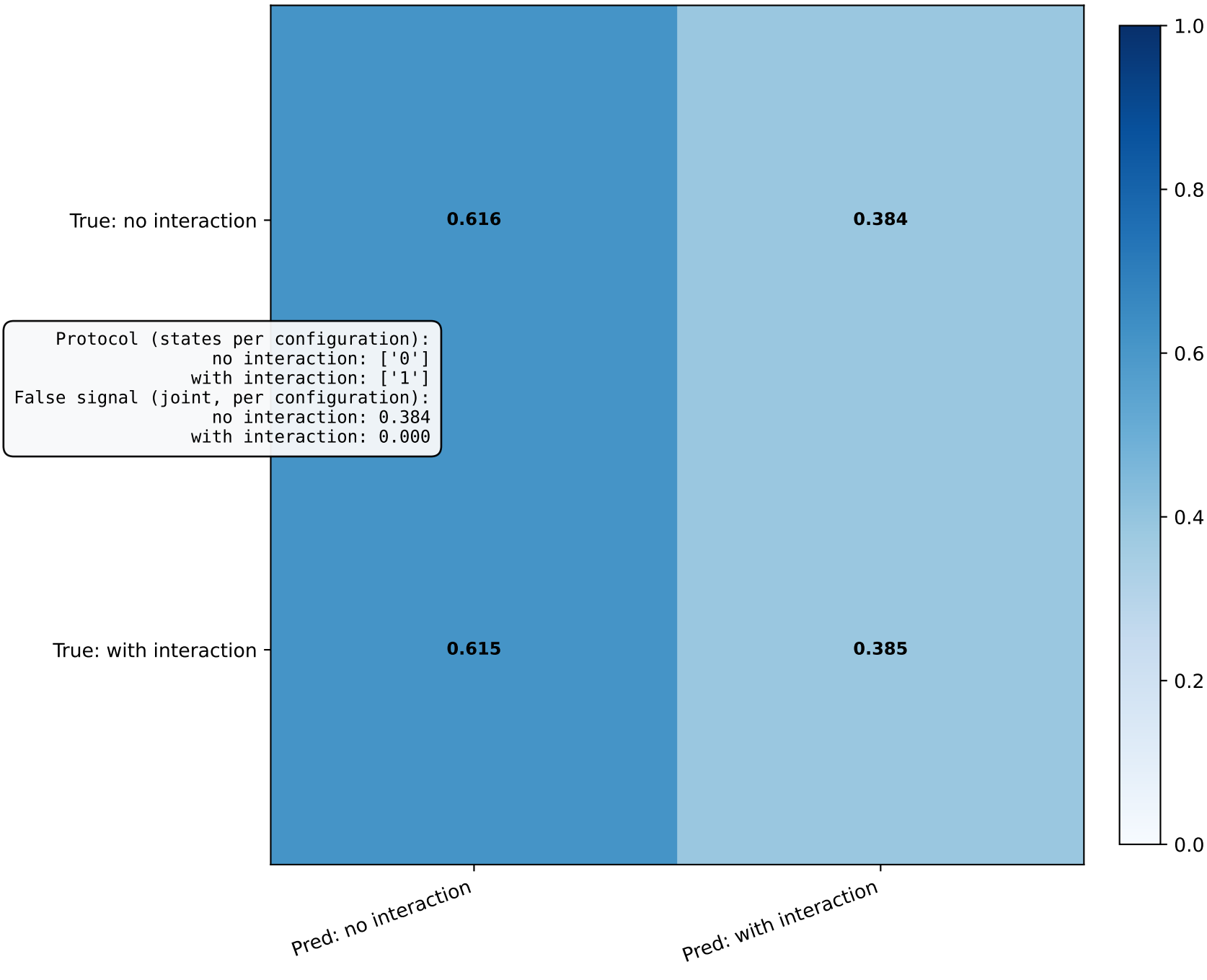
Confusion Matrix
