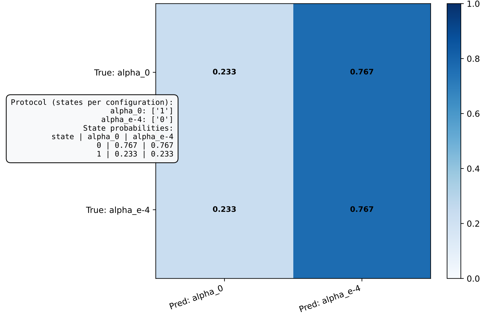
Confusion Matrix
