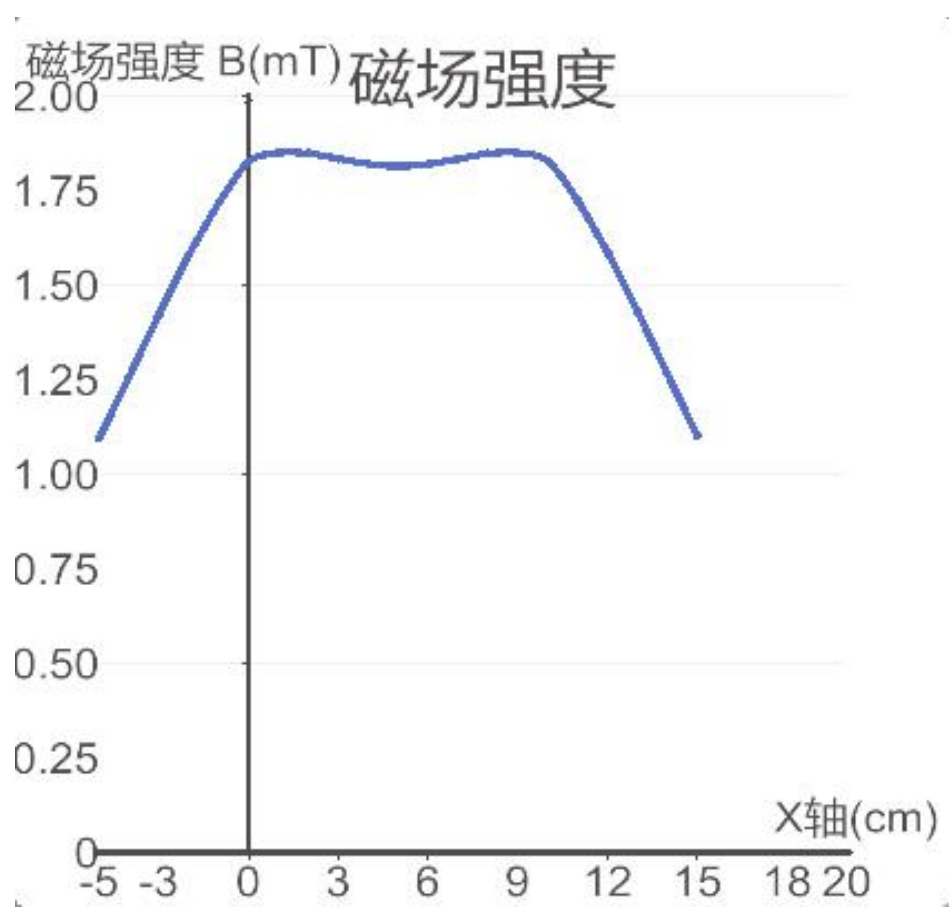
二、磁场空间分布图 ( f = 50.0 Hz, I = 1.0 mA, d = 10.0 cm)
