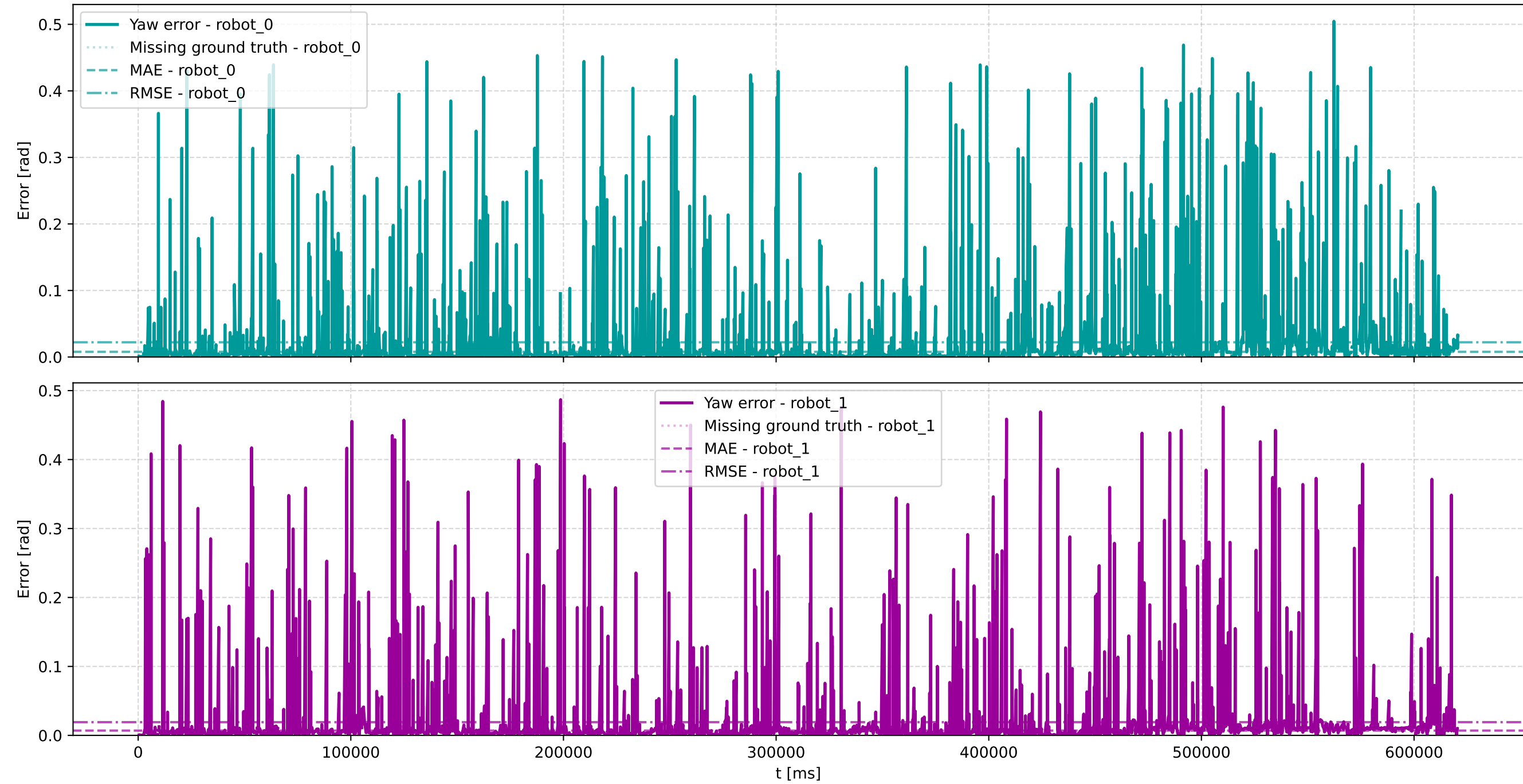
Yaw Error with MAE & RMSE
