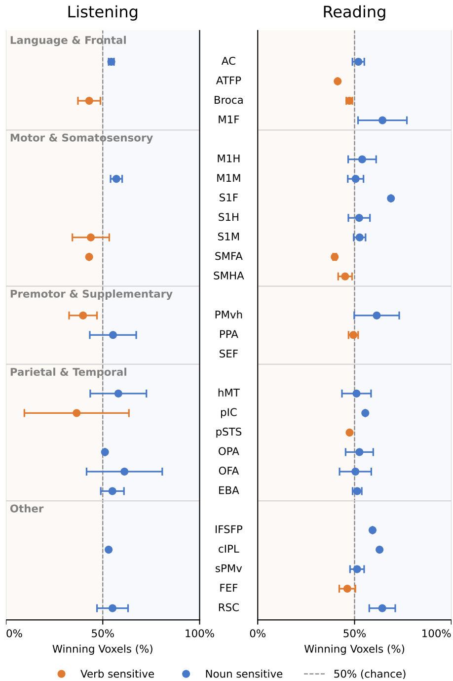
Figure 4. Relative reliance on nouns versus verbs across regions of interest (ROIs). Points indicate the proportion of the total performance drop within each ROI attributable to masking the preferred word class. Values are computed by summing the voxel-wise performance decrements (baseline > masked condition) for nouns and verbs, and expressing each as a percentage of the total combined decrement. The dashed line at 50% represents equal reliance on both grammatical classes. Values further from the center indicate a stronger magnitude-weighted dominance. Error bars represent \pm 1 standard deviation across n subjects.
