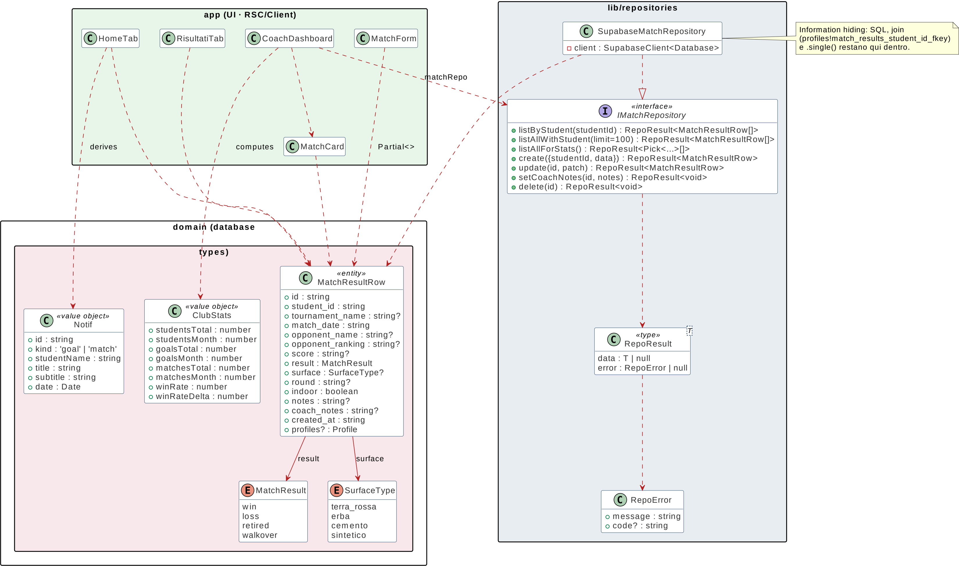
Tennis Club Bellusco — Class Diagram Iter. 3 (vista Logical)
