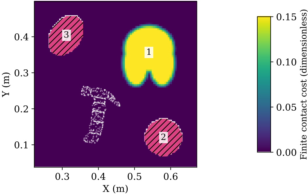
XY slice at Z = 0.015 m
