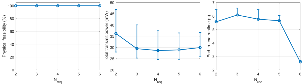
Figure 2: Physical feasibility, total transmit power, and runtime versus the required sensing-cluster size. Error bars show the 10th–90th percentile interval.
