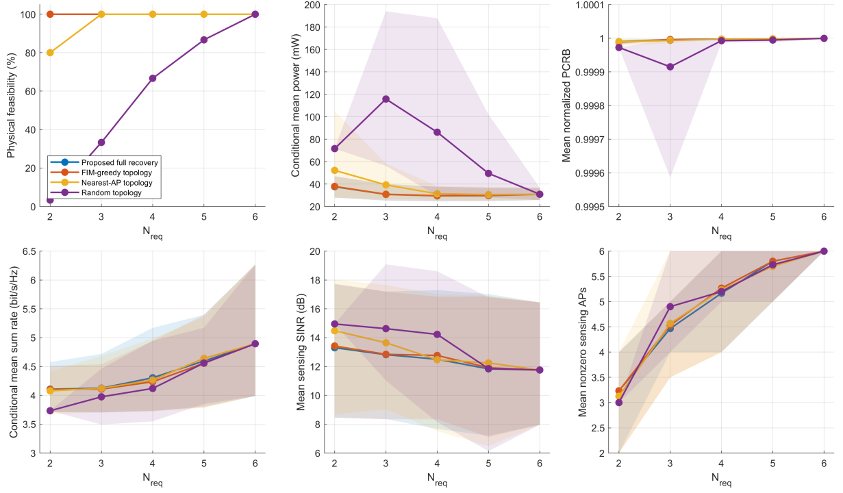
Figure 4: Thirty-seed comparison of physical association and recovery methods versus the required sensing-cluster size. Power, sum rate, sensing SINR, and the number of active sensing APs are conditional on physical feasibility; shaded bands denote the 10th–90th percentile interval.
