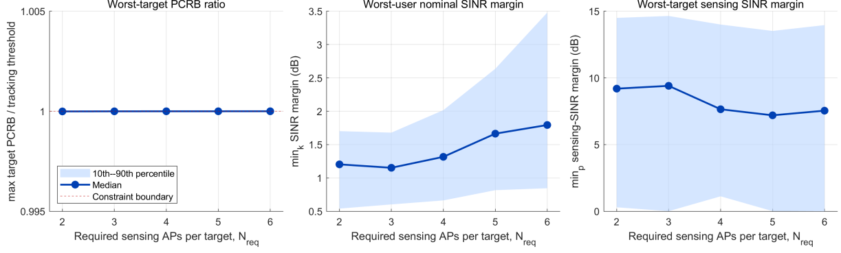
Figure 3: QoS statistics versus sensing-cluster size. Shaded regions denote the 10th–90th percentile interval across feasible trials.
