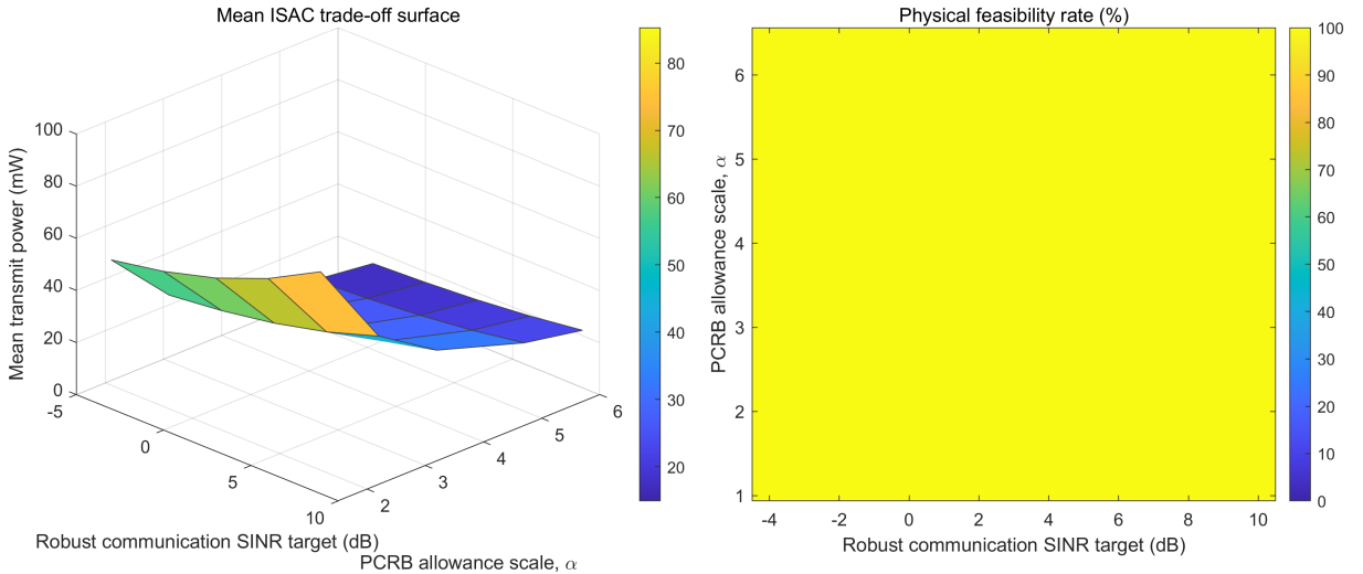
Figure 6: Statistical communication–sensing trade-off surface and physical feasibility heat map over five common seeds.
