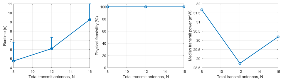
Figure 5: Runtime and physical feasibility versus total antenna dimension.
