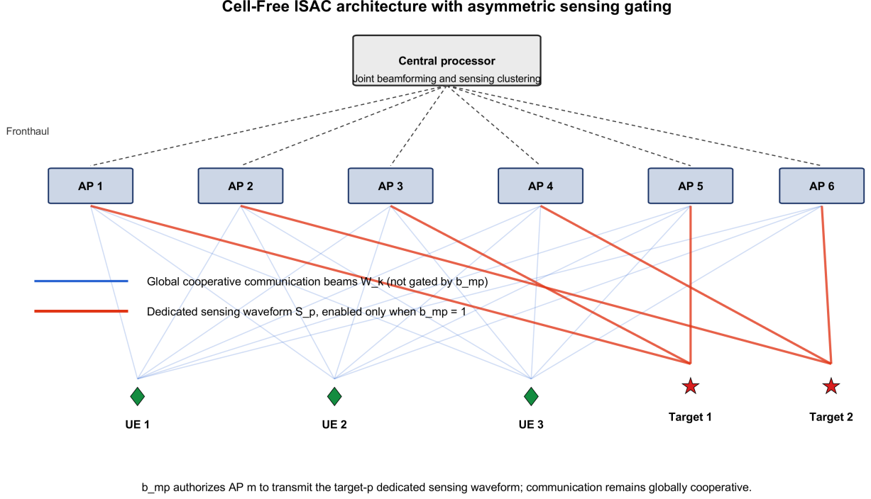
Figure 1: Cell-Free ISAC architecture. Global communication beamforming is not gated by b_{mp} , whereas each selected AP–target pair radiates a nonzero target-specific dedicated sensing component.
