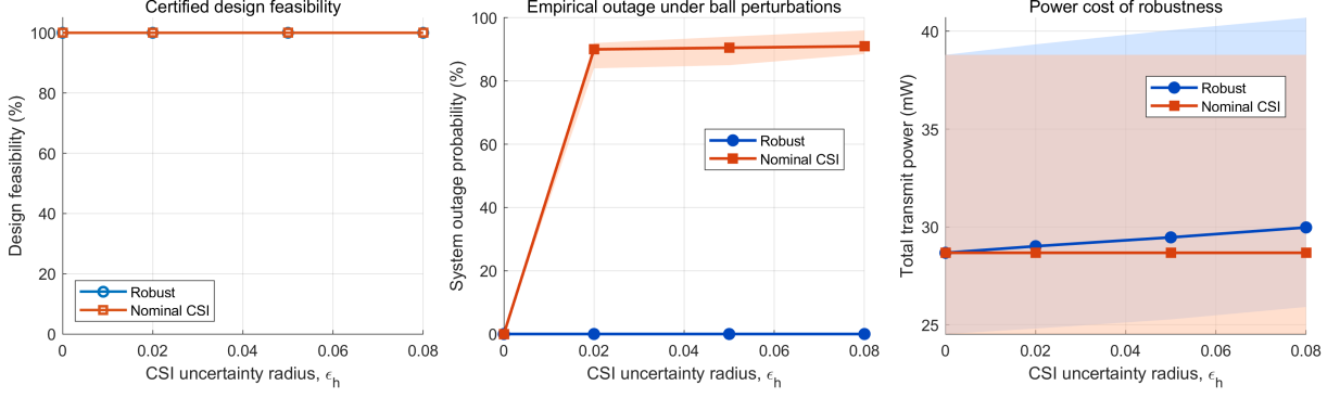
Figure 7: Robust and nominal CSI designs under ball-bounded channel perturbations.
