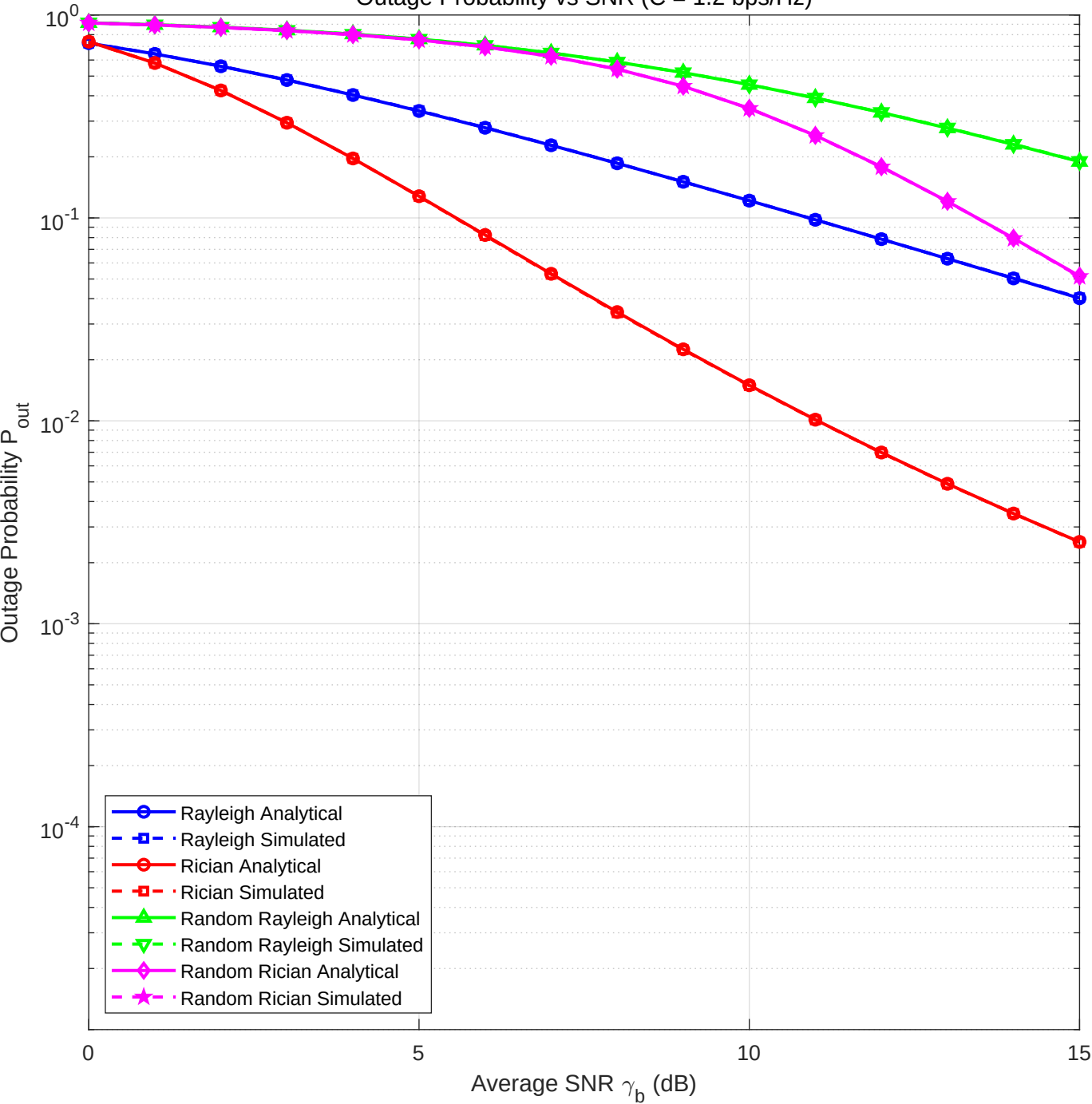
Outage Probability vs SNR ( C = 1.2 bps/Hz)
