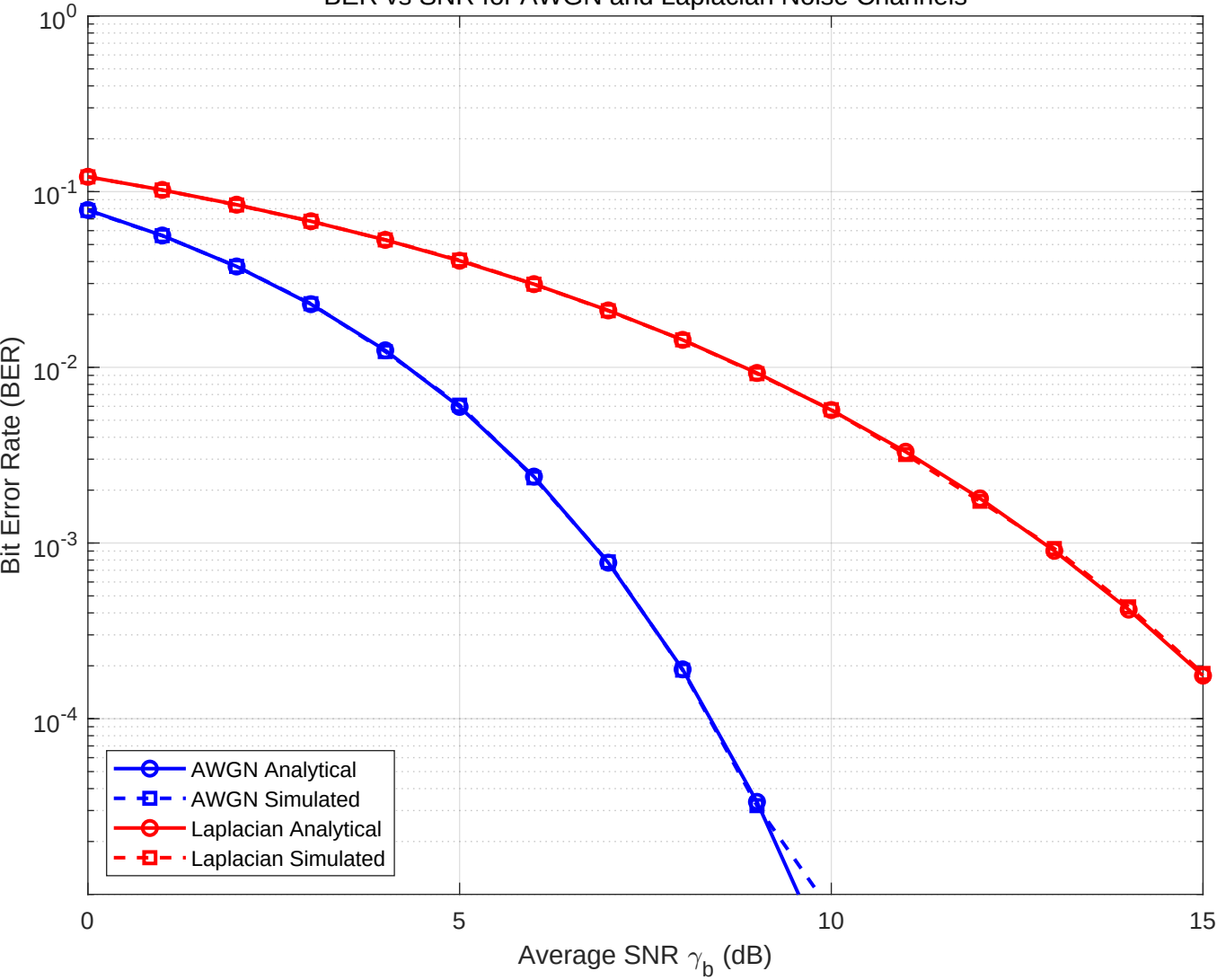
BER vs SNR for AWGN and Laplacian Noise Channels
