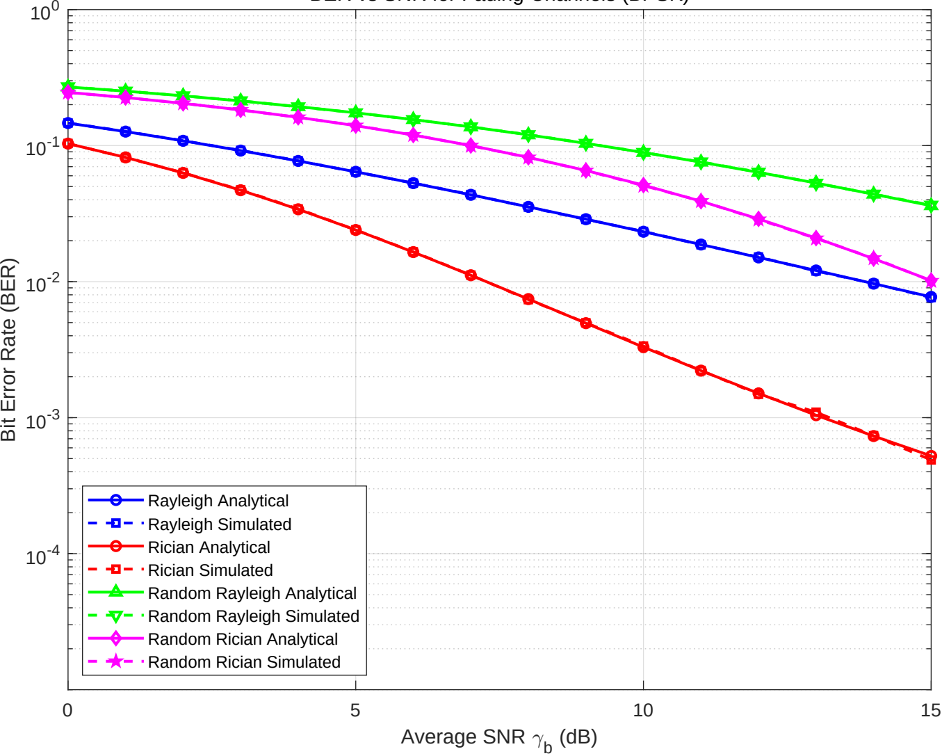
BER vs SNR for Fading Channels (BPSK)
