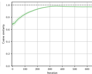
Update Similarity
