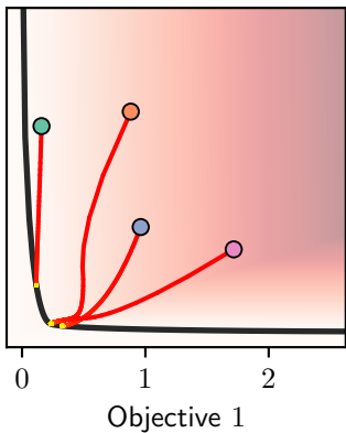
\mathcal{A}_{\text{UPGrad}} (ours)
