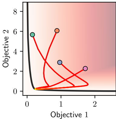
\mathcal{A}_{\text{Mean}}
