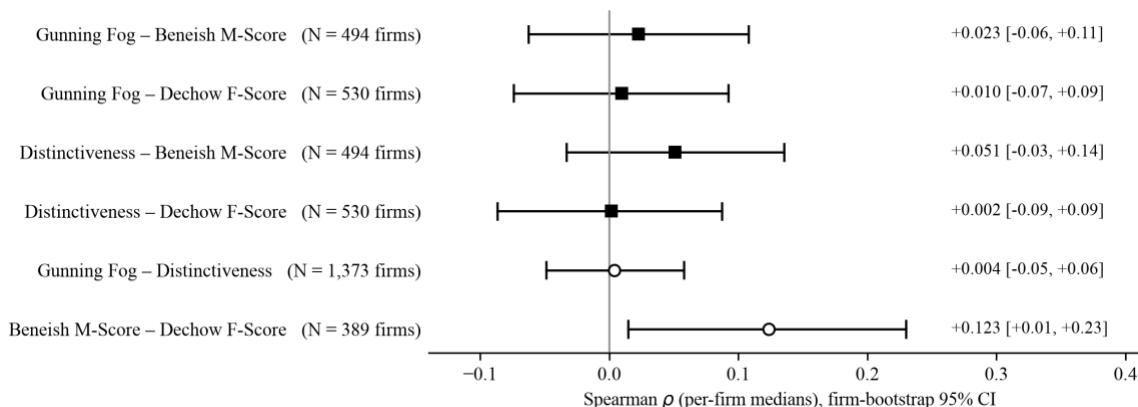
Figure 4. Firm-level Spearman correlations with 95% confidence intervals
