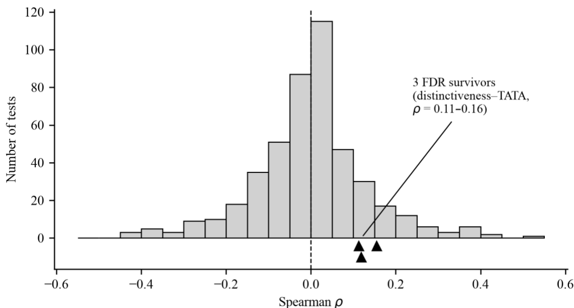
Figure 3. Distribution of Spearman \rho across all 460 tests
