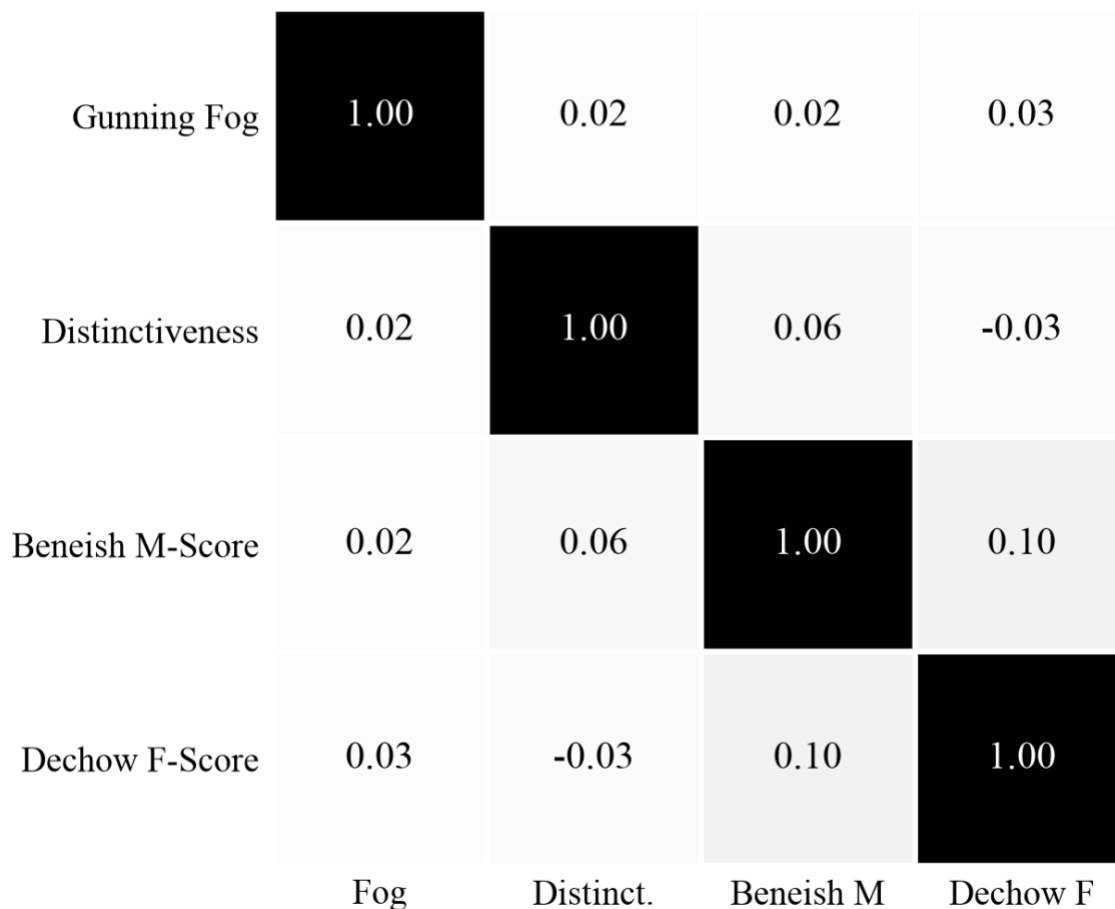
Figure 2. Correlation matrix visualization
