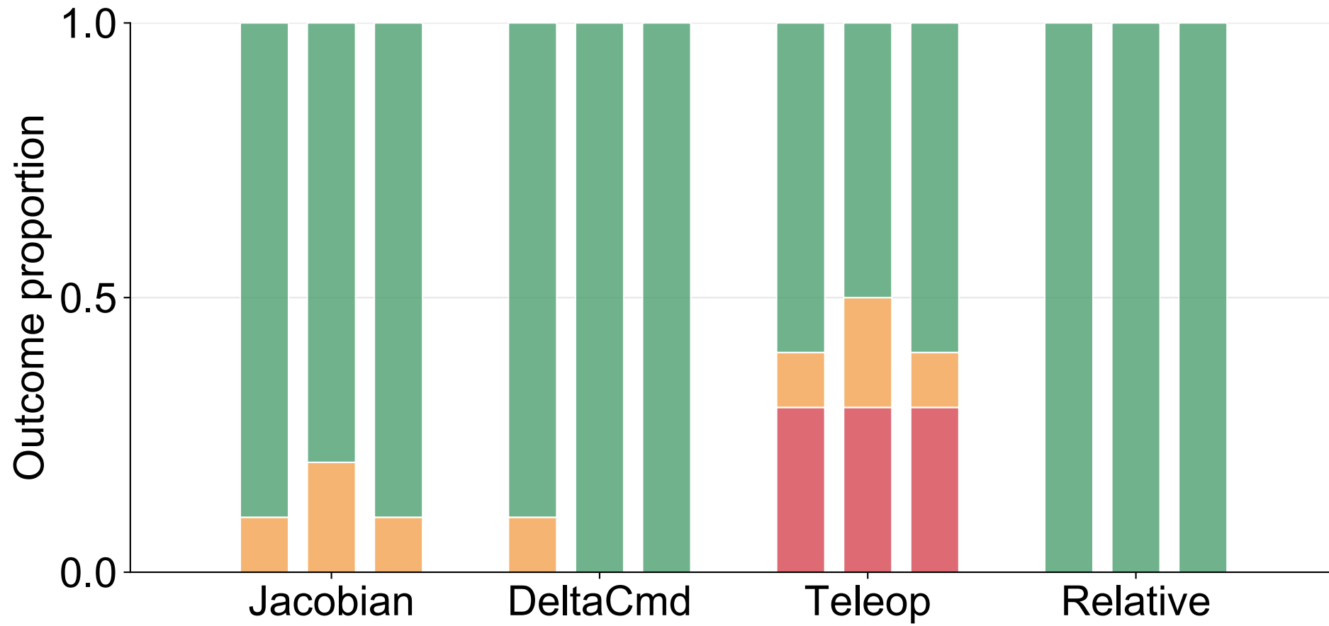
Drill Task: Post-takeover outcome (Attempts 1–3)
