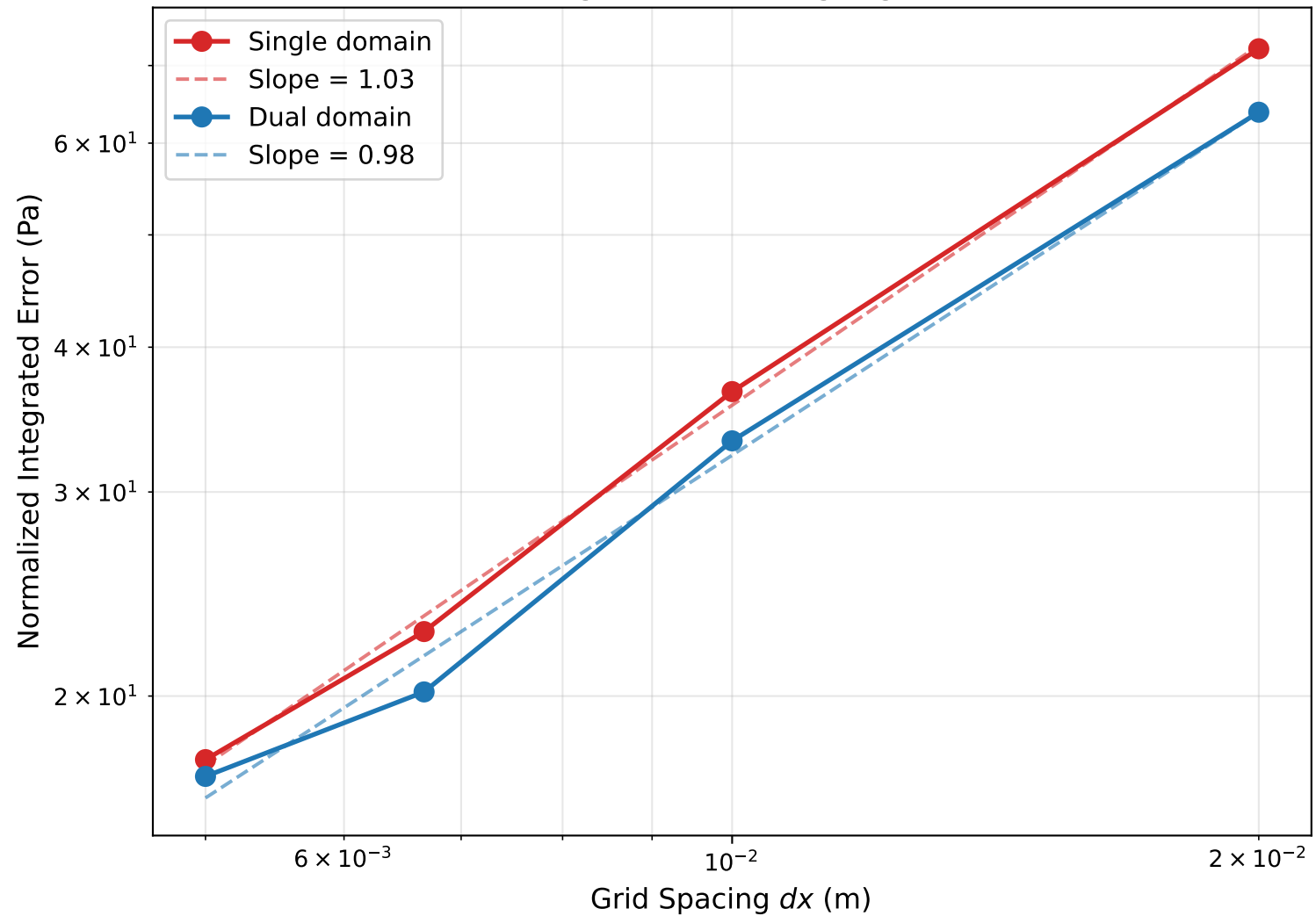
Convergence Rate (log-log scale)
